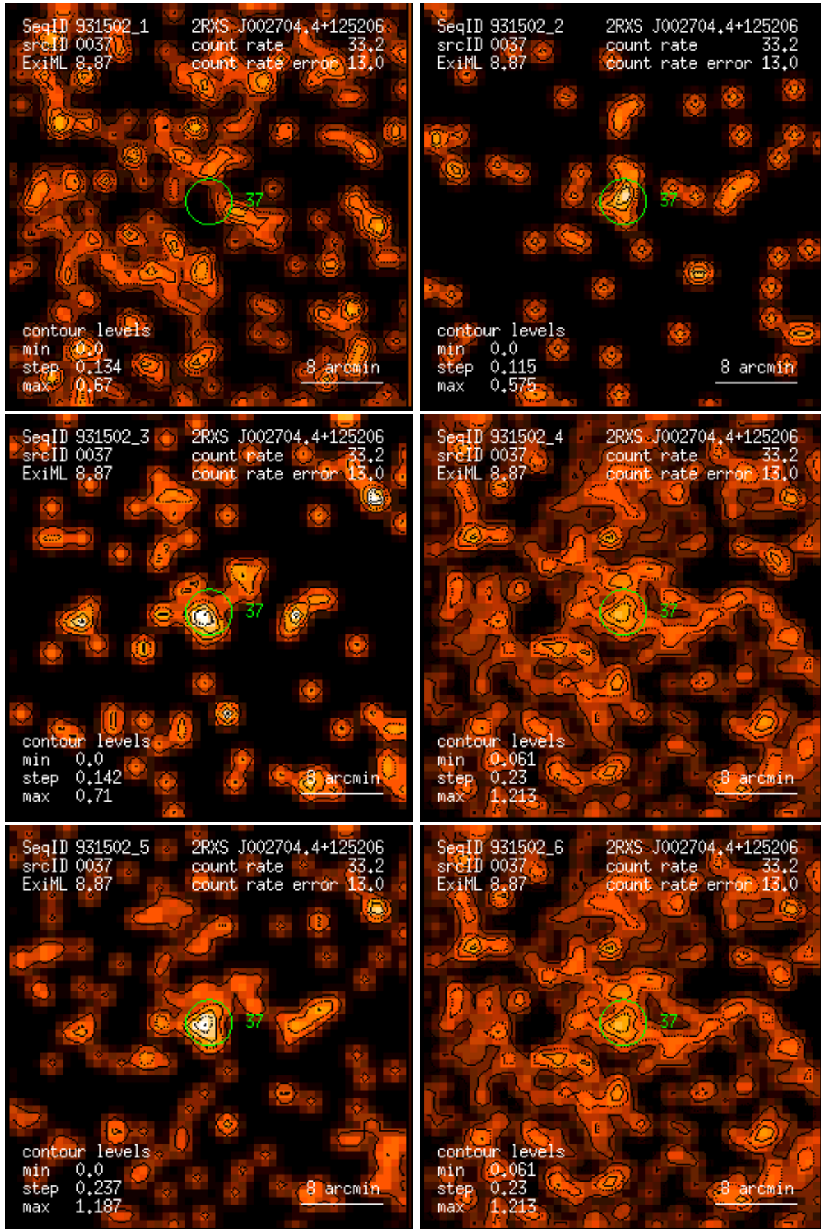
Figure 37: RASS 931502: detection 0037: band rate images, Gaussian filter: (1) PSPC channels 11 – 41, (2) 52 – 90, (3) 91 – 201, (4) 11 – 235, (5) 52 – 201, (6) 11 – 201. Broad band rates in counts/ks. Band rate contour levels in counts/ks/arcmin 2 .
