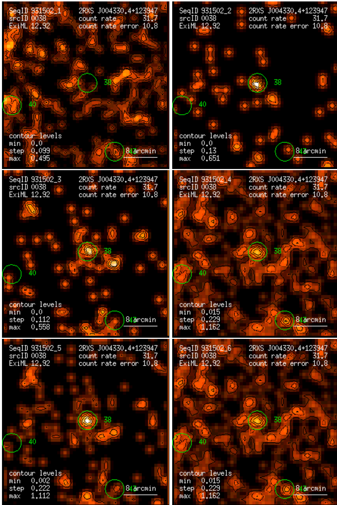
Figure 38: RASS 931502: detection 0038: band rate images, Gaussian filter: (1) PSPC channels 11 – 41, (2) 52 – 90, (3) 91 – 201, (4) 11 – 235, (5) 52 – 201, (6) 11 – 201. Broad band rates in counts/ks. Band rate contour levels in counts/ks/arcmin 2 .
