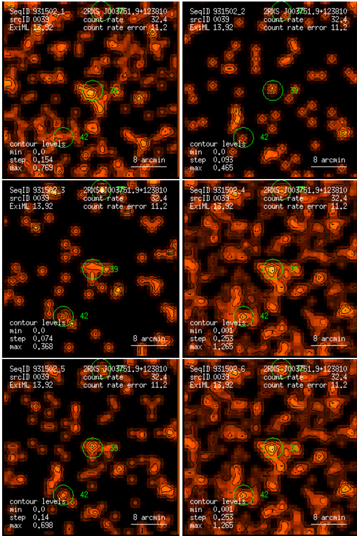
Figure 39: RASS 931502: detection 0039: band rate images, Gaussian filter: (1) PSPC channels 11 – 41, (2) 52 – 90, (3) 91 – 201, (4) 11 – 235, (5) 52 – 201, (6) 11 – 201. Broad band rates in counts/ks. Band rate contour levels in counts/ks/arcmin 2 .
