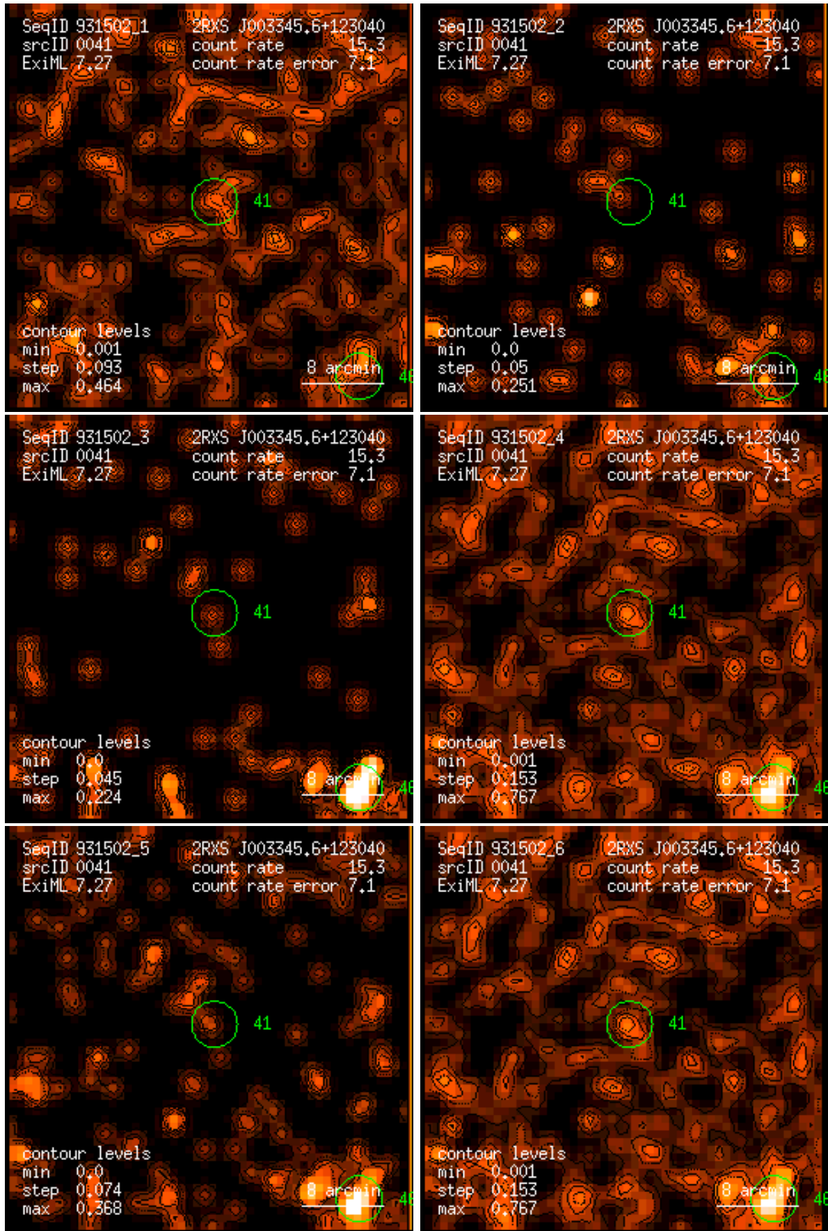
Figure 41: RASS 931502: detection 0041: band rate images, Gaussian filter: (1) PSPC channels 11 – 41, (2) 52 – 90, (3) 91 – 201, (4) 11 – 235, (5) 52 – 201, (6) 11 – 201. Broad band rates in counts/ks. Band rate contour levels in counts/ks/arcmin 2 .
