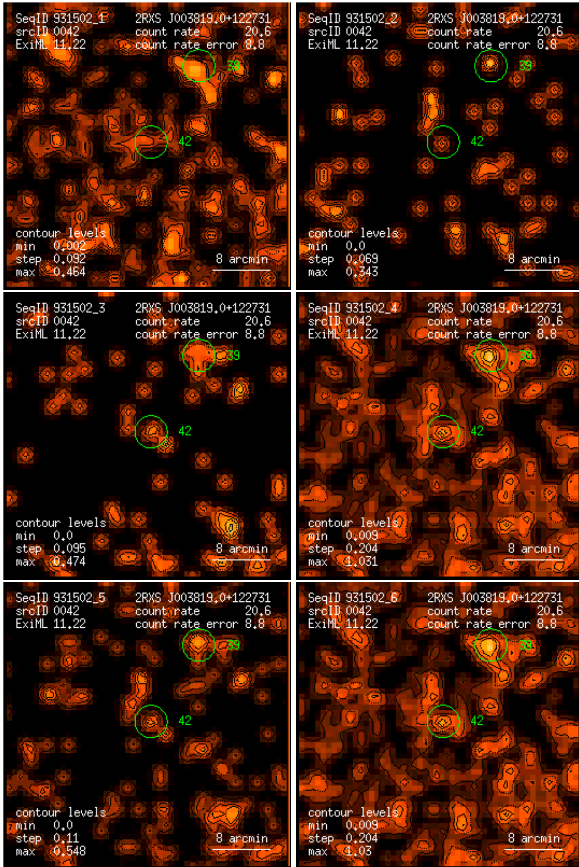
Figure 42: RASS 931502: detection 0042: band rate images, Gaussian filter: (1) PSPC channels 11 – 41, (2) 52 – 90, (3) 91 – 201, (4) 11 – 235, (5) 52 – 201, (6) 11 – 201. Broad band rates in counts/ks. Band rate contour levels in counts/ks/arcmin 2 .
