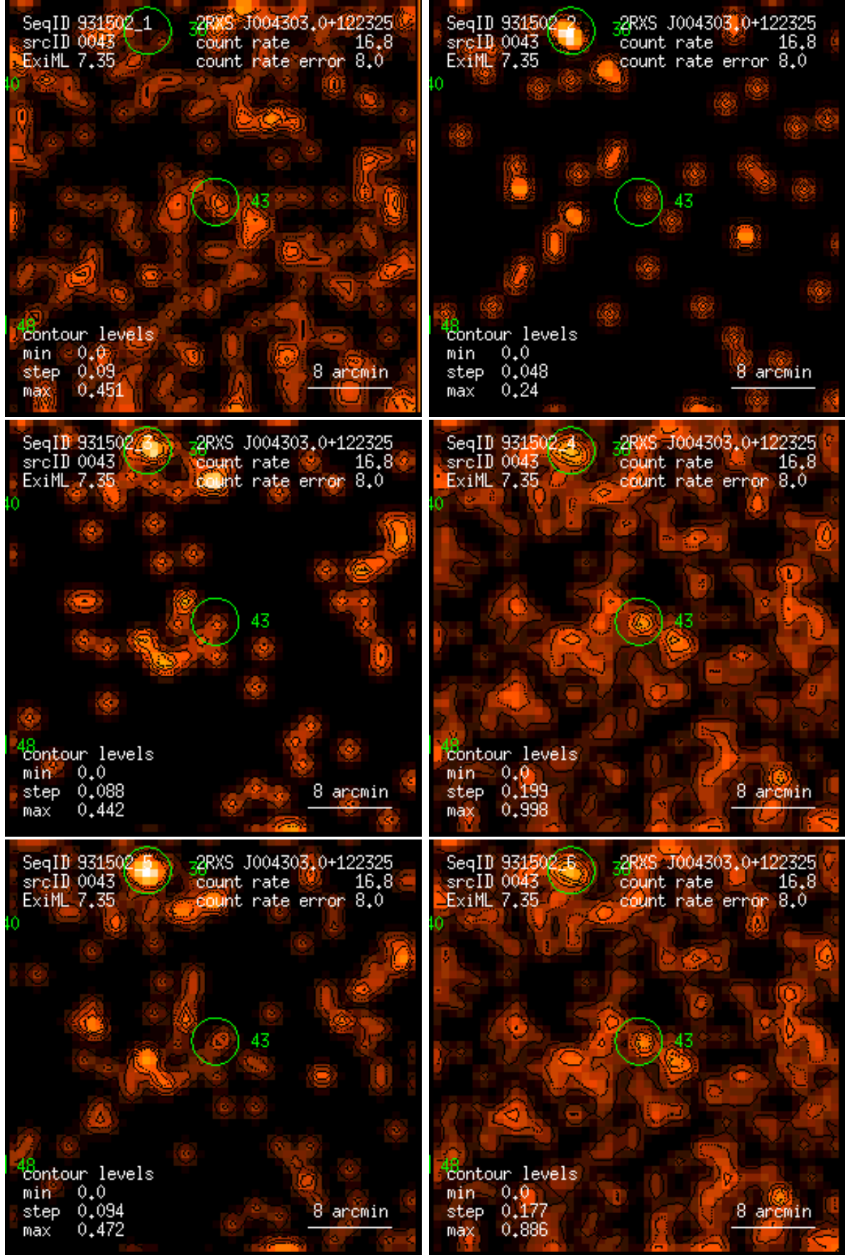
Figure 43: RASS 931502: detection 0043: band rate images, Gaussian filter: (1) PSPC channels 11 – 41, (2) 52 – 90, (3) 91 – 201, (4) 11 – 235, (5) 52 – 201, (6) 11 – 201. Broad band rates in counts/ks. Band rate contour levels in counts/ks/arcmin 2 .
