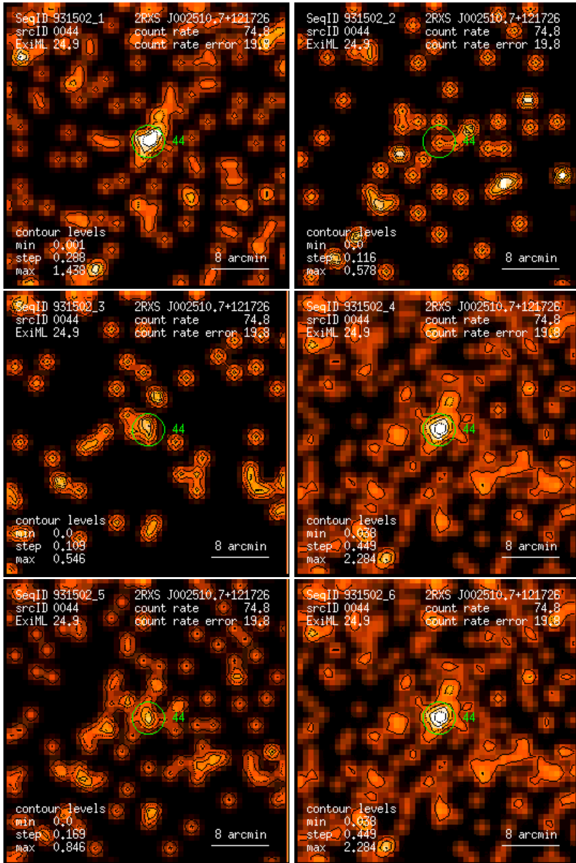
Figure 44: RASS 931502: detection 0044: band rate images, Gaussian filter: (1) PSPC channels 11 – 41, (2) 52 – 90, (3) 91 – 201, (4) 11 – 235, (5) 52 – 201, (6) 11 – 201. Broad band rates in counts/ks. Band rate contour levels in counts/ks/arcmin 2 .
