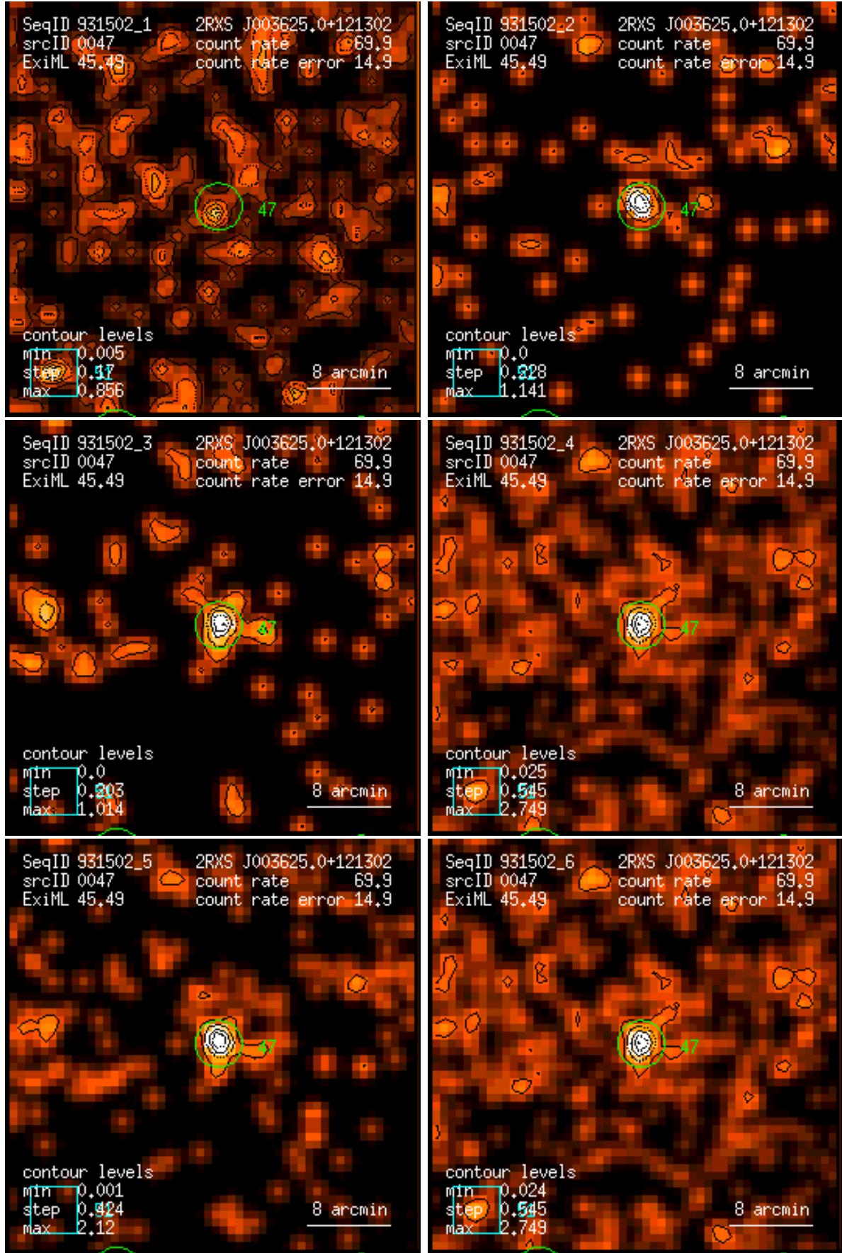
Figure 47: RASS 931502: detection 0047: band rate images, Gaussian filter: (1) PSPC channels 11 – 41, (2) 52 – 90, (3) 91 – 201, (4) 11 – 235, (5) 52 – 201, (6) 11 – 201. Broad band rates in counts/ks. Band rate contour levels in counts/ks/arcmin 2 .
