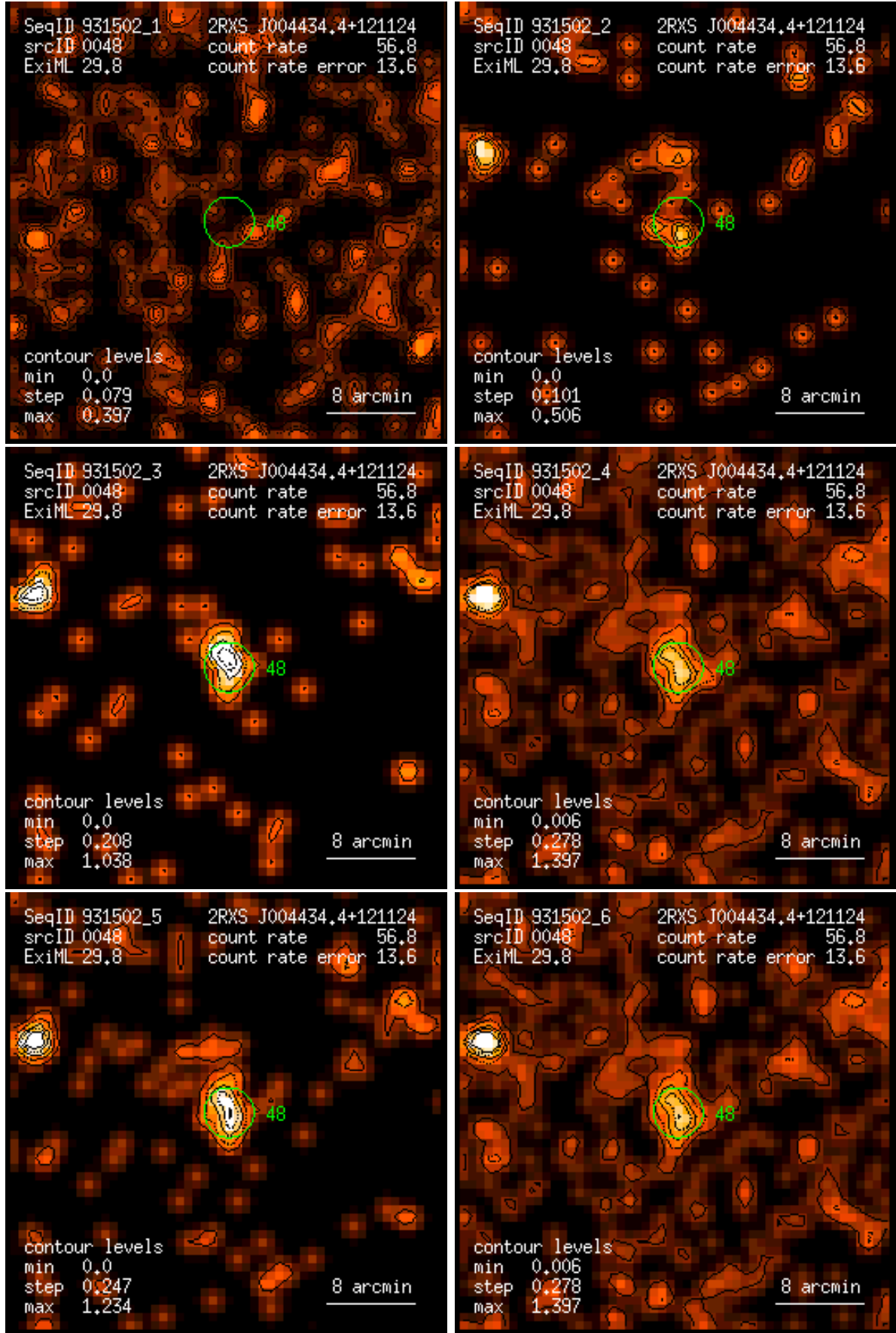
Figure 48: RASS 931502: detection 0048: band rate images, Gaussian filter: (1) PSPC channels 11 – 41, (2) 52 – 90, (3) 91 – 201, (4) 11 – 235, (5) 52 – 201, (6) 11 – 201. Broad band rates in counts/ks. Band rate contour levels in counts/ks/arcmin 2 .
