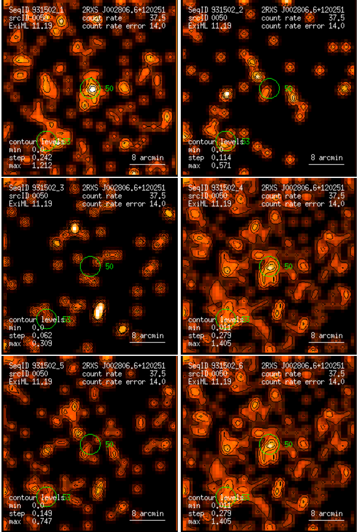
Figure 50: RASS 931502: detection 0050: band rate images, Gaussian filter: (1) PSPC channels 11 – 41, (2) 52 – 90, (3) 91 – 201, (4) 11 – 235, (5) 52 – 201, (6) 11 – 201. Broad band rates in counts/ks. Band rate contour levels in counts/ks/arcmin 2 .
