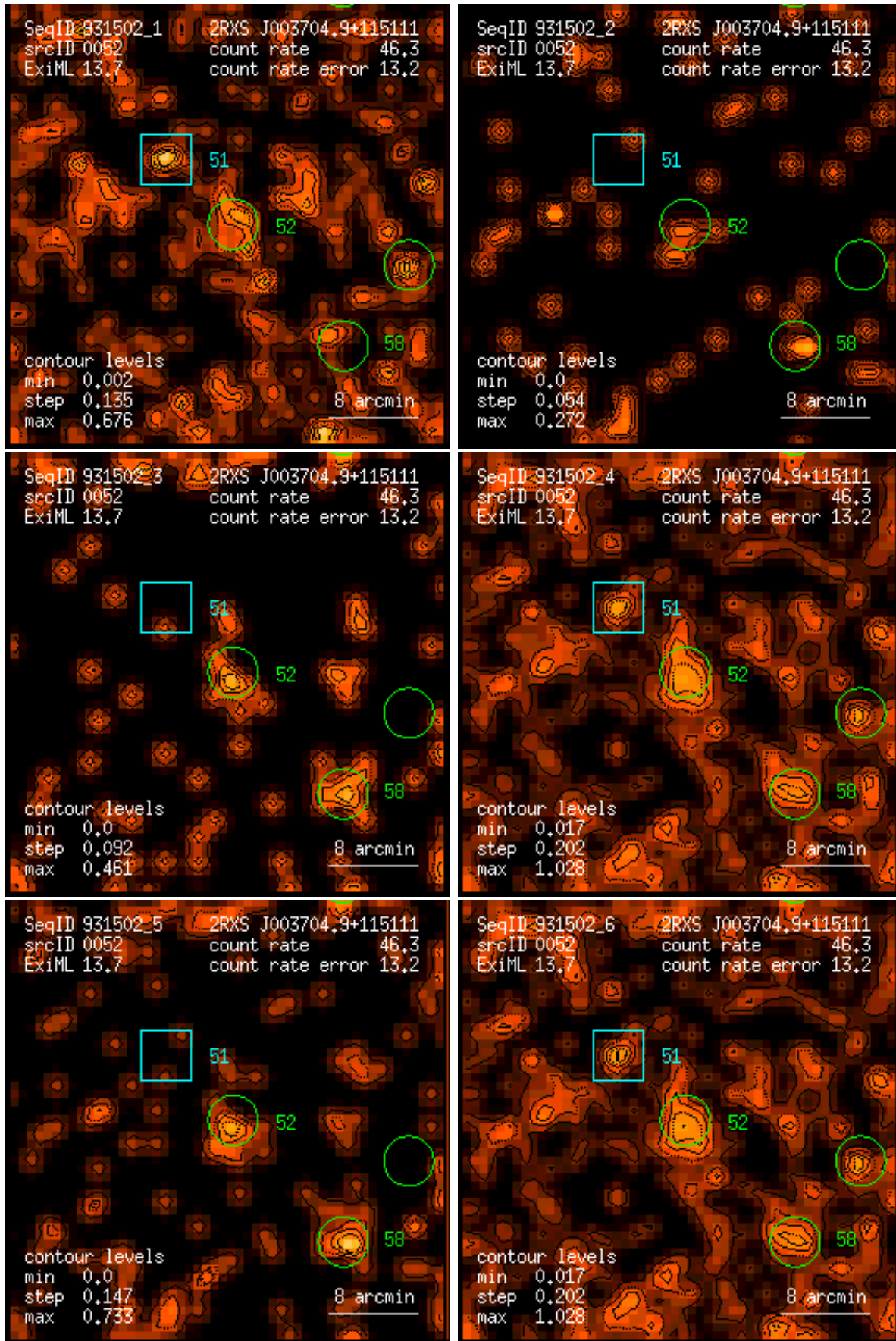
Figure 52: RASS 931502: detection 0052: band rate images, Gaussian filter: (1) PSPC channels 11 – 41, (2) 52 – 90, (3) 91 – 201, (4) 11 – 235, (5) 52 – 201, (6) 11 – 201. Broad band rates in counts/ks. Band rate contour levels in counts/ks/arcmin 2 .
