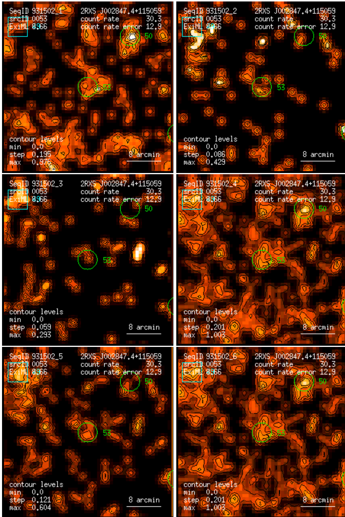
Figure 53: RASS 931502: detection 0053: band rate images, Gaussian filter: (1) PSPC channels 11 – 41, (2) 52 – 90, (3) 91 – 201, (4) 11 – 235, (5) 52 – 201, (6) 11 – 201. Broad band rates in counts/ks. Band rate contour levels in counts/ks/arcmin 2 .
