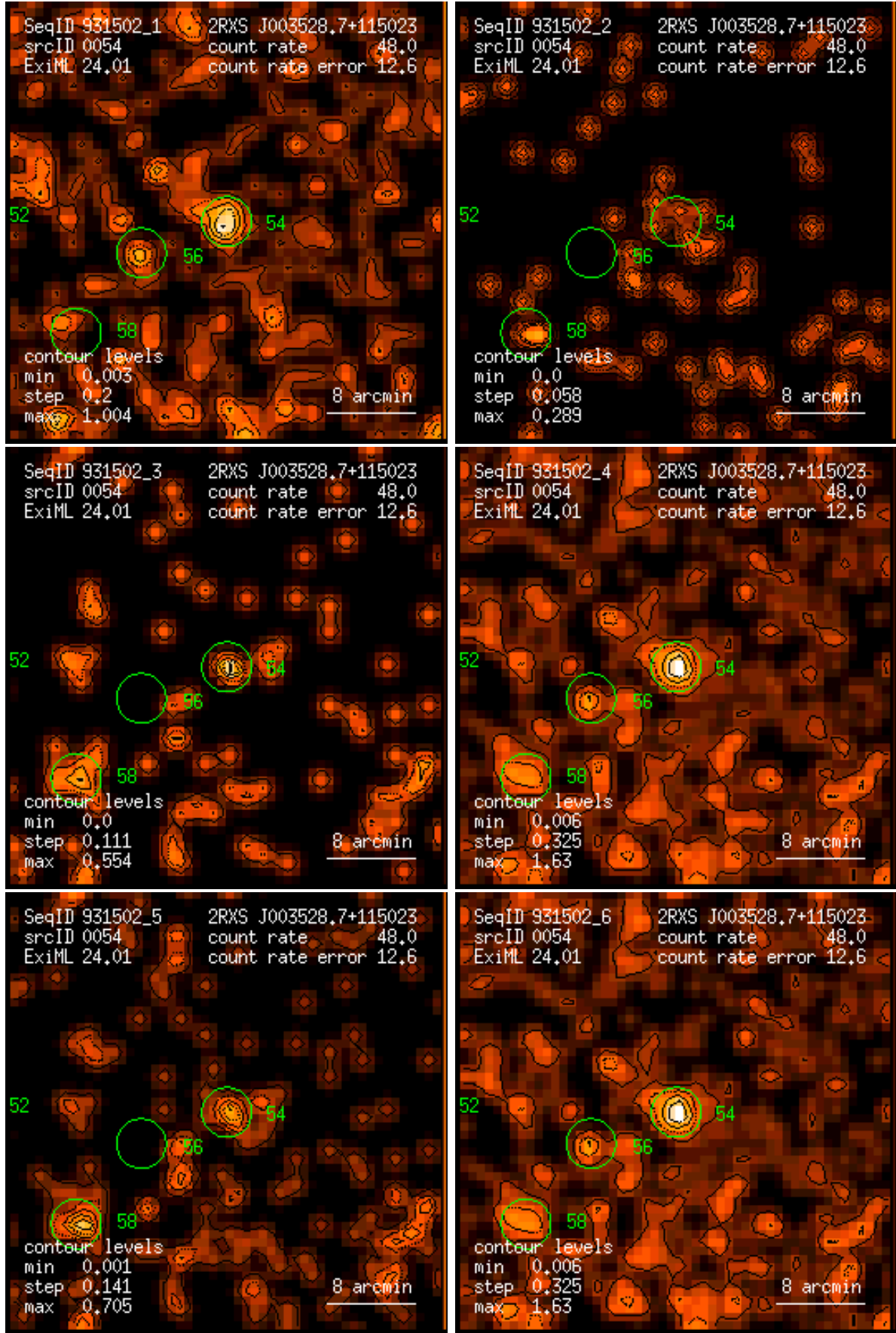
Figure 54: RASS 931502: detection 0054: band rate images, Gaussian filter: (1) PSPC channels 11 – 41, (2) 52 – 90, (3) 91 – 201, (4) 11 – 235, (5) 52 – 201, (6) 11 – 201. Broad band rates in counts/ks. Band rate contour levels in counts/ks/arcmin 2 .
