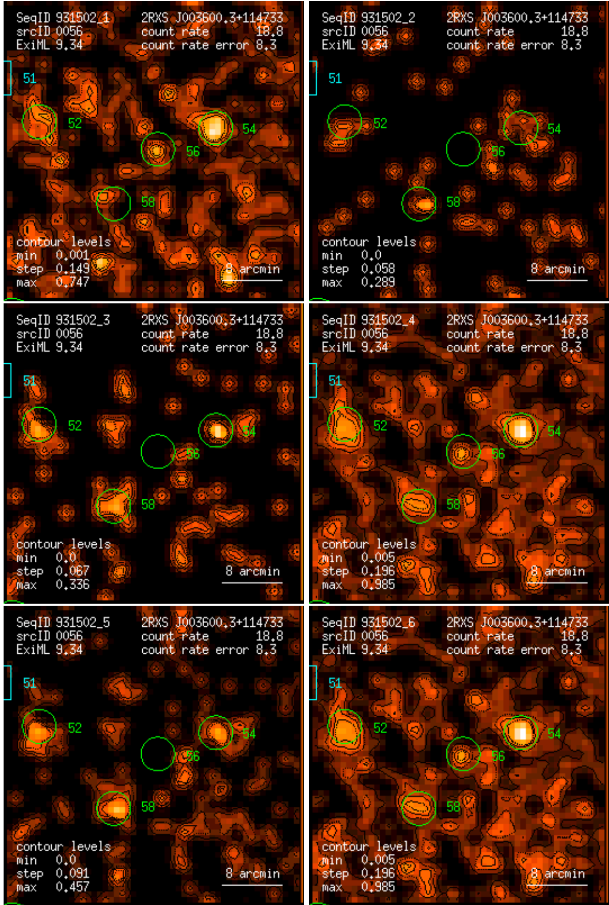
Figure 56: RASS 931502: detection 0056: band rate images, Gaussian filter: (1) PSPC channels 11 – 41, (2) 52 – 90, (3) 91 – 201, (4) 11 – 235, (5) 52 – 201, (6) 11 – 201. Broad band rates in counts/ks. Band rate contour levels in counts/ks/arcmin 2 .
