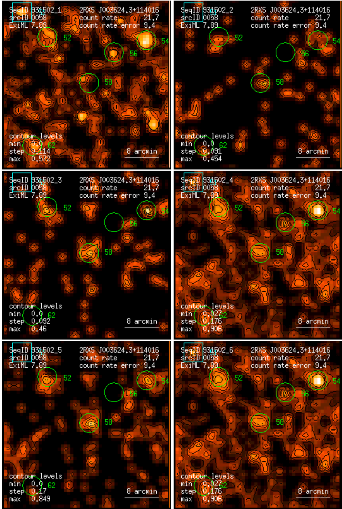
Figure 58: RASS 931502: detection 0058: band rate images, Gaussian filter: (1) PSPC channels 11 – 41, (2) 52 – 90, (3) 91 – 201, (4) 11 – 235, (5) 52 – 201, (6) 11 – 201. Broad band rates in counts/ks. Band rate contour levels in counts/ks/arcmin 2 .
