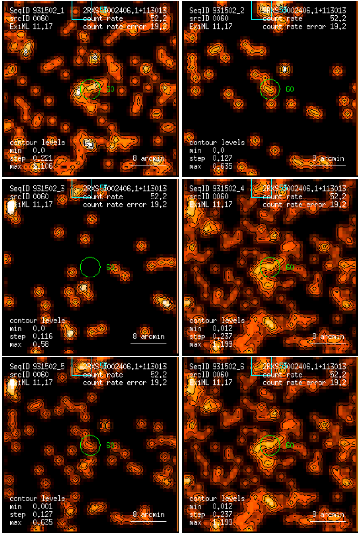
Figure 60: RASS 931502: detection 0060: band rate images, Gaussian filter: (1) PSPC channels 11 – 41, (2) 52 – 90, (3) 91 – 201, (4) 11 – 235, (5) 52 – 201, (6) 11 – 201. Broad band rates in counts/ks. Band rate contour levels in counts/ks/arcmin 2 .
