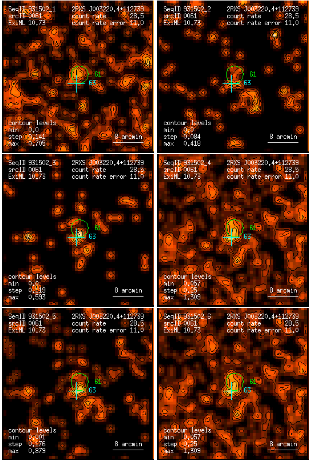
Figure 61: RASS 931502: detection 0061: band rate images, Gaussian filter: (1) PSPC channels 11 – 41, (2) 52 – 90, (3) 91 – 201, (4) 11 – 235, (5) 52 – 201, (6) 11 – 201. Broad band rates in counts/ks. Band rate contour levels in counts/ks/arcmin 2 .
