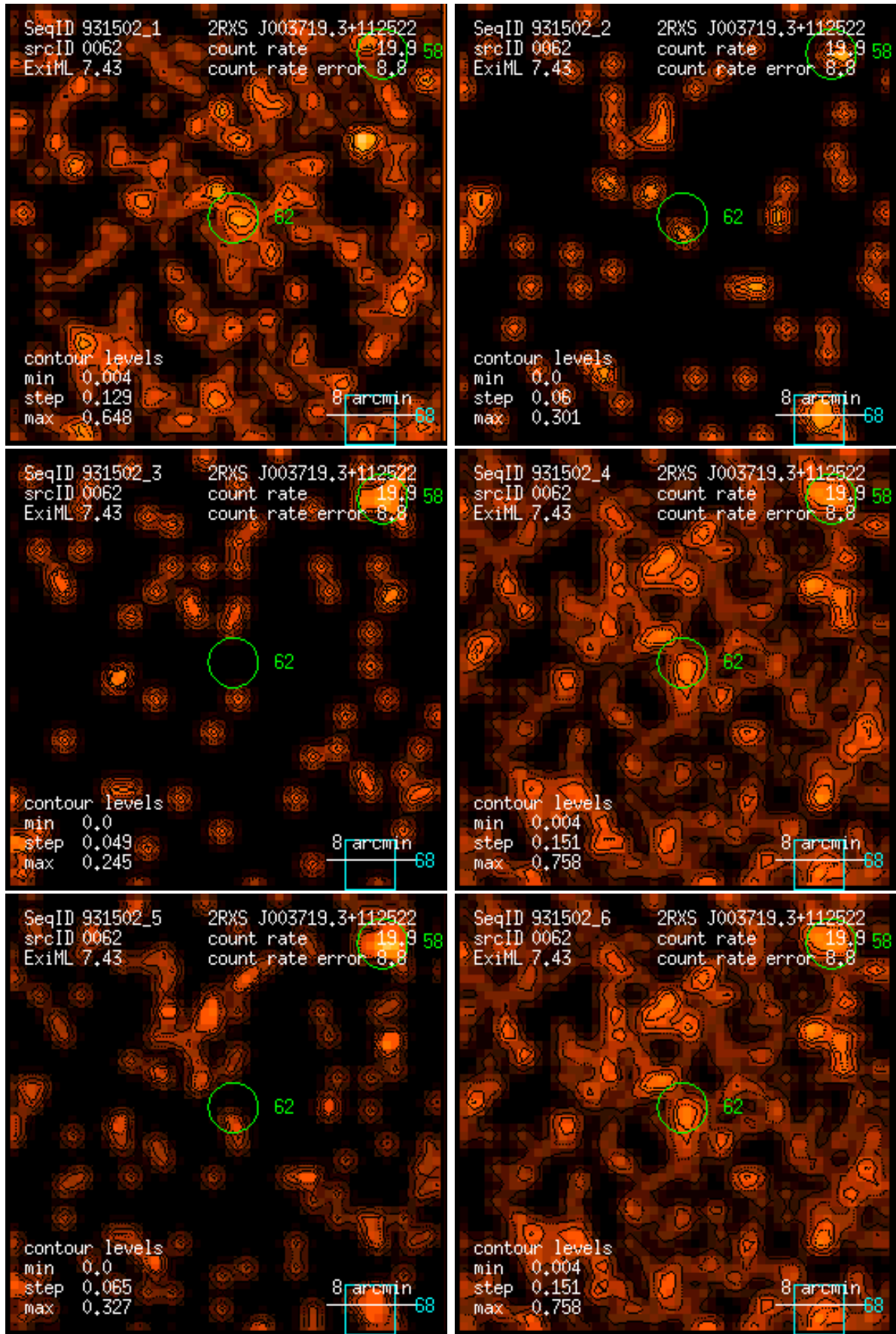
Figure 62: RASS 931502: detection 0062: band rate images, Gaussian filter: (1) PSPC channels 11 – 41, (2) 52 – 90, (3) 91 – 201, (4) 11 – 235, (5) 52 – 201, (6) 11 – 201. Broad band rates in counts/ks. Band rate contour levels in counts/ks/arcmin 2 .
