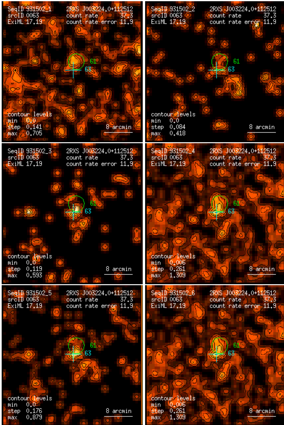
Figure 63: RASS 931502: detection 0063: band rate images, Gaussian filter: (1) PSPC channels 11 – 41, (2) 52 – 90, (3) 91 – 201, (4) 11 – 235, (5) 52 – 201, (6) 11 – 201. Broad band rates in counts/ks. Band rate contour levels in counts/ks/arcmin 2 .
