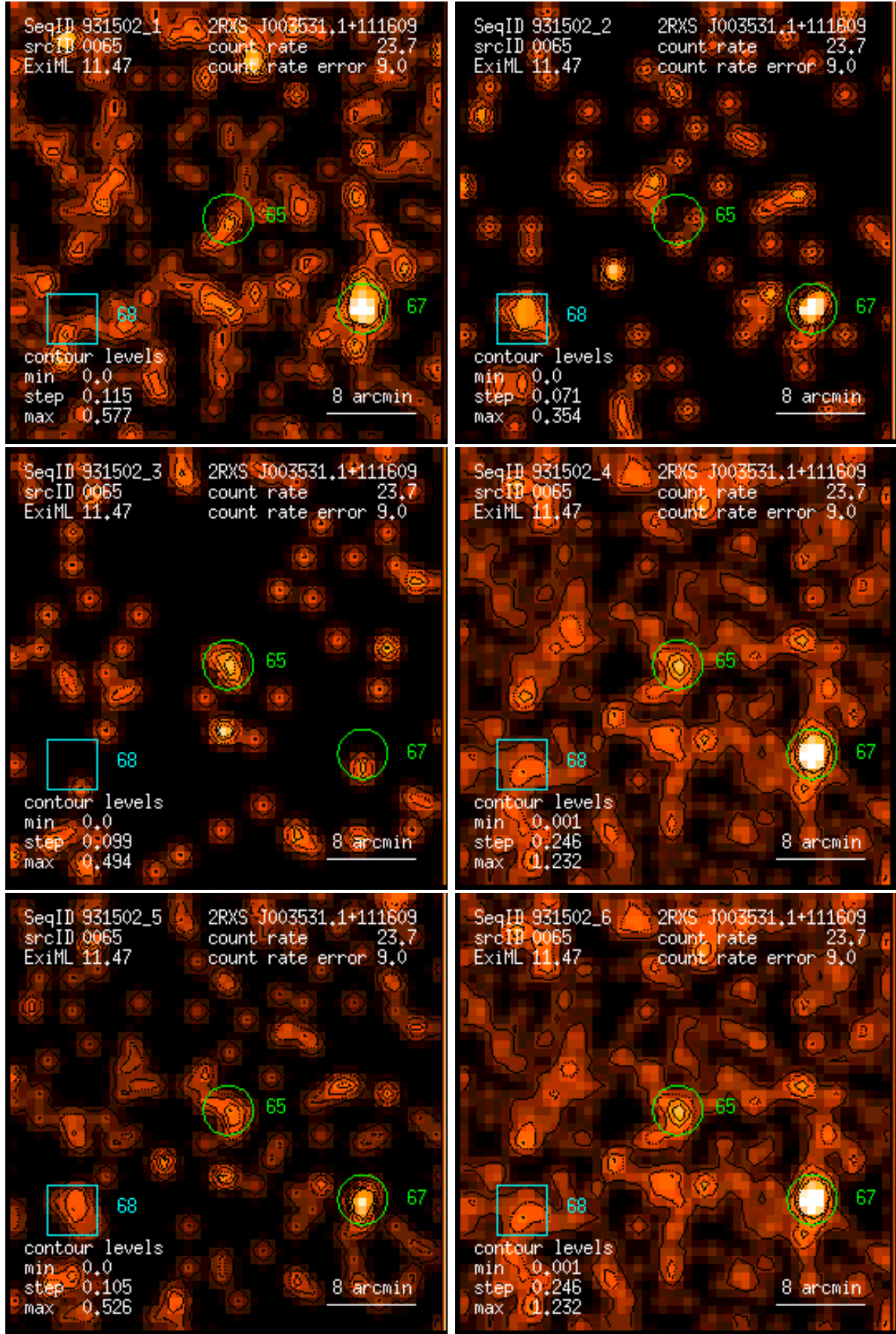
Figure 65: RASS 931502: detection 0065: band rate images, Gaussian filter: (1) PSPC channels 11 – 41, (2) 52 – 90, (3) 91 – 201, (4) 11 – 235, (5) 52 – 201, (6) 11 – 201. Broad band rates in counts/ks. Band rate contour levels in counts/ks/arcmin 2 .
