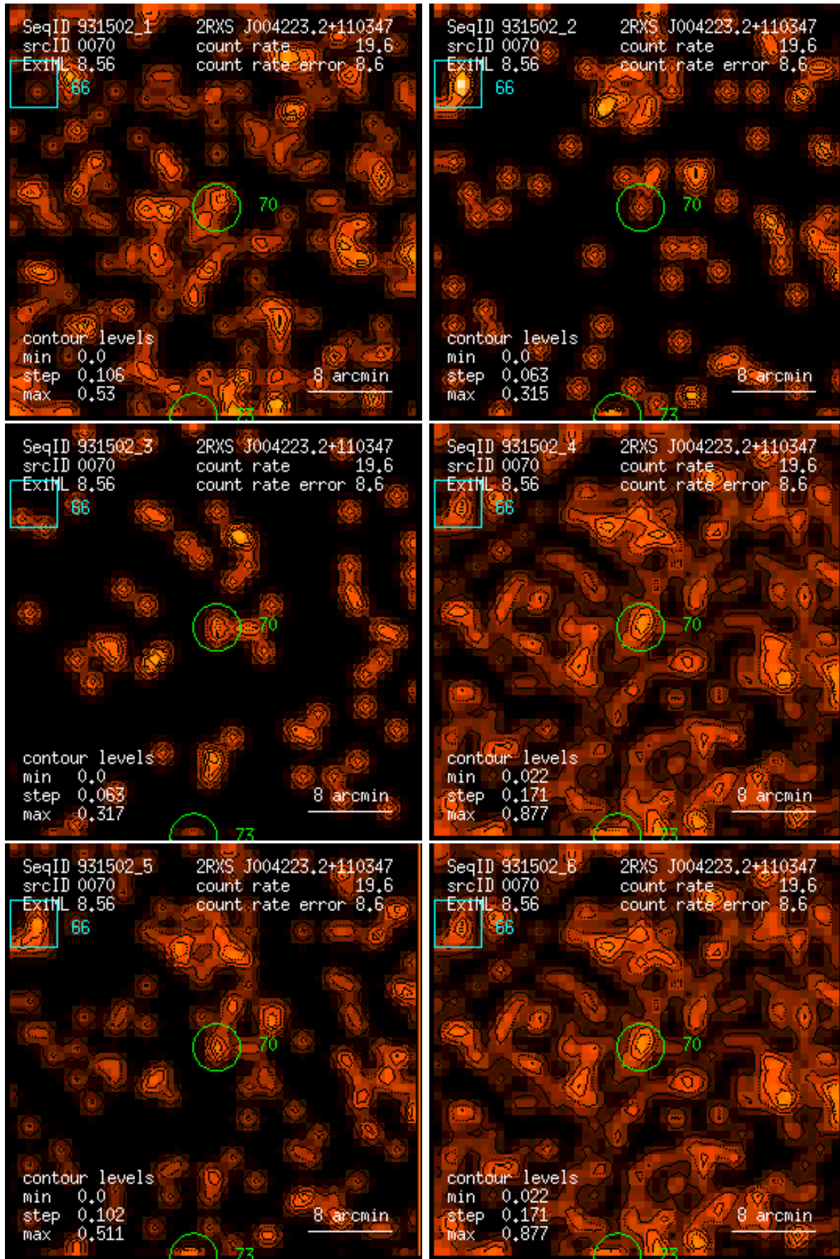
Figure 70: RASS 931502: detection 0070: band rate images, Gaussian filter: (1) PSPC channels 11 – 41, (2) 52 – 90, (3) 91 – 201, (4) 11 – 235, (5) 52 – 201, (6) 11 – 201. Broad band rates in counts/ks. Band rate contour levels in counts/ks/arcmin 2 .
