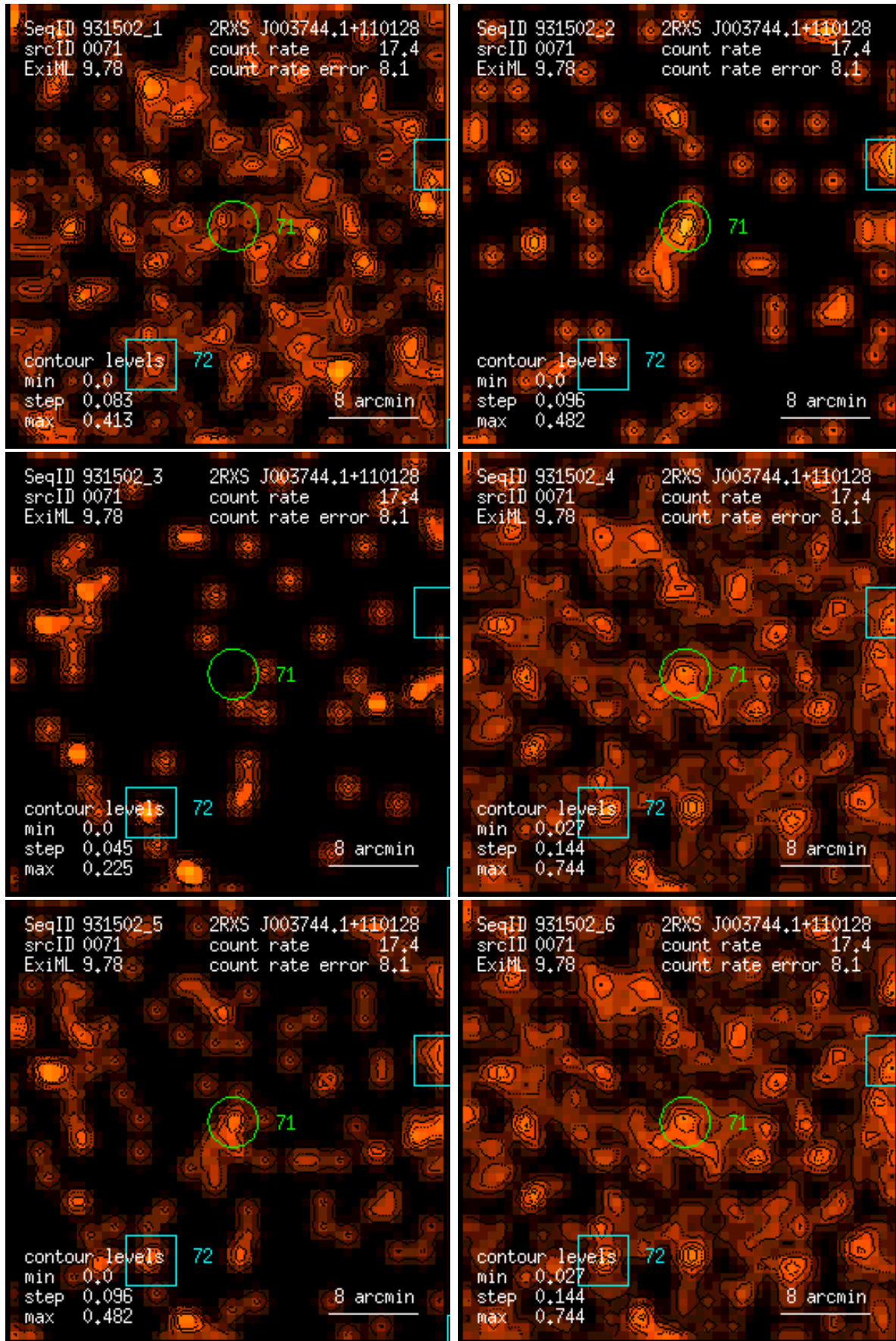
Figure 71: RASS 931502: detection 0071: band rate images, Gaussian filter: (1) PSPP channels 11 – 41, (2) 52 – 90, (3) 91 – 201, (4) 11 – 235, (5) 52 – 201, (6) 11 – 201. Broad band rates in counts/ks. Band rate contour levels in counts/ks/arcmin 2 .
