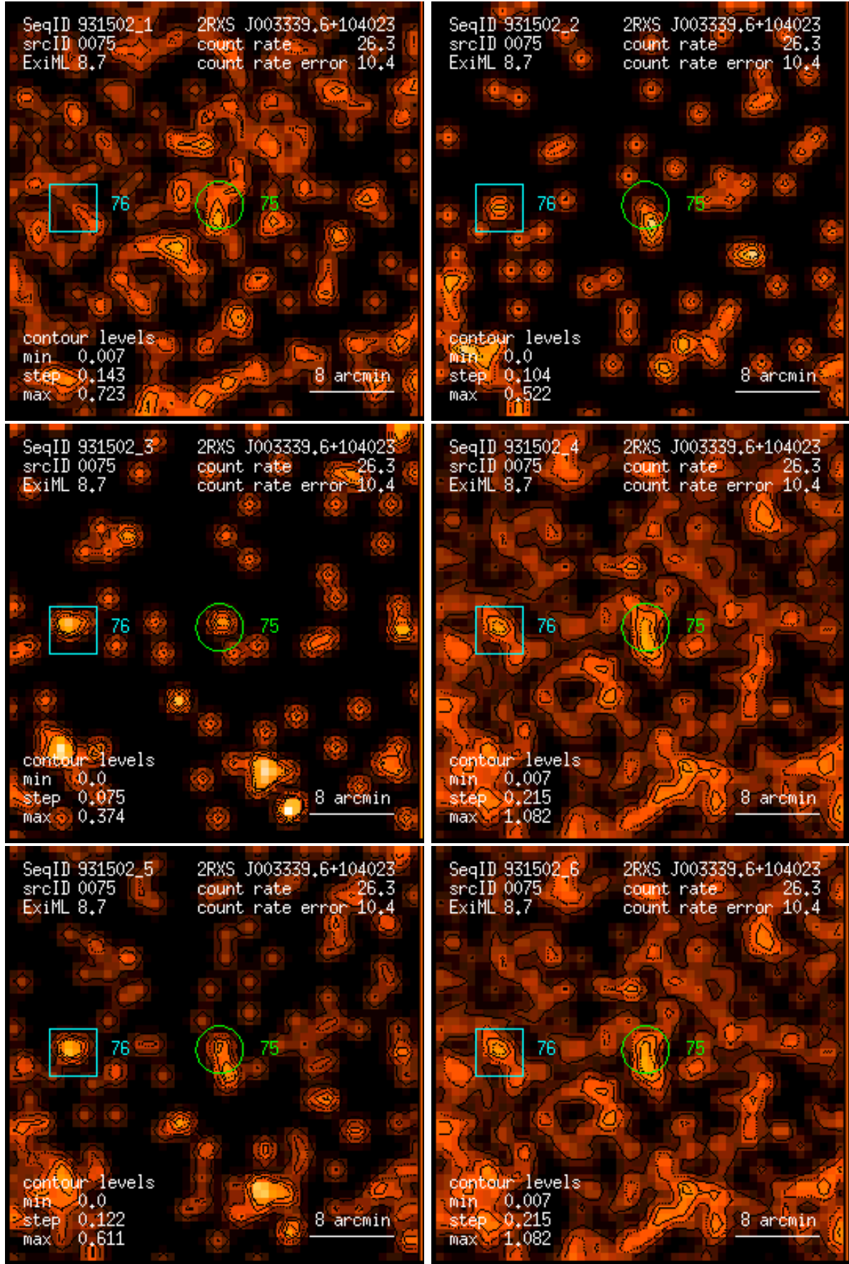
Figure 75: RASS 931502: detection 0075: band rate images, Gaussian filter: (1) PSPC channels 11 – 41, (2) 52 – 90, (3) 91 – 201, (4) 11 – 235, (5) 52 – 201, (6) 11 – 201. Broad band rates in counts/ks. Band rate contour levels in counts/ks/arcmin 2 .
