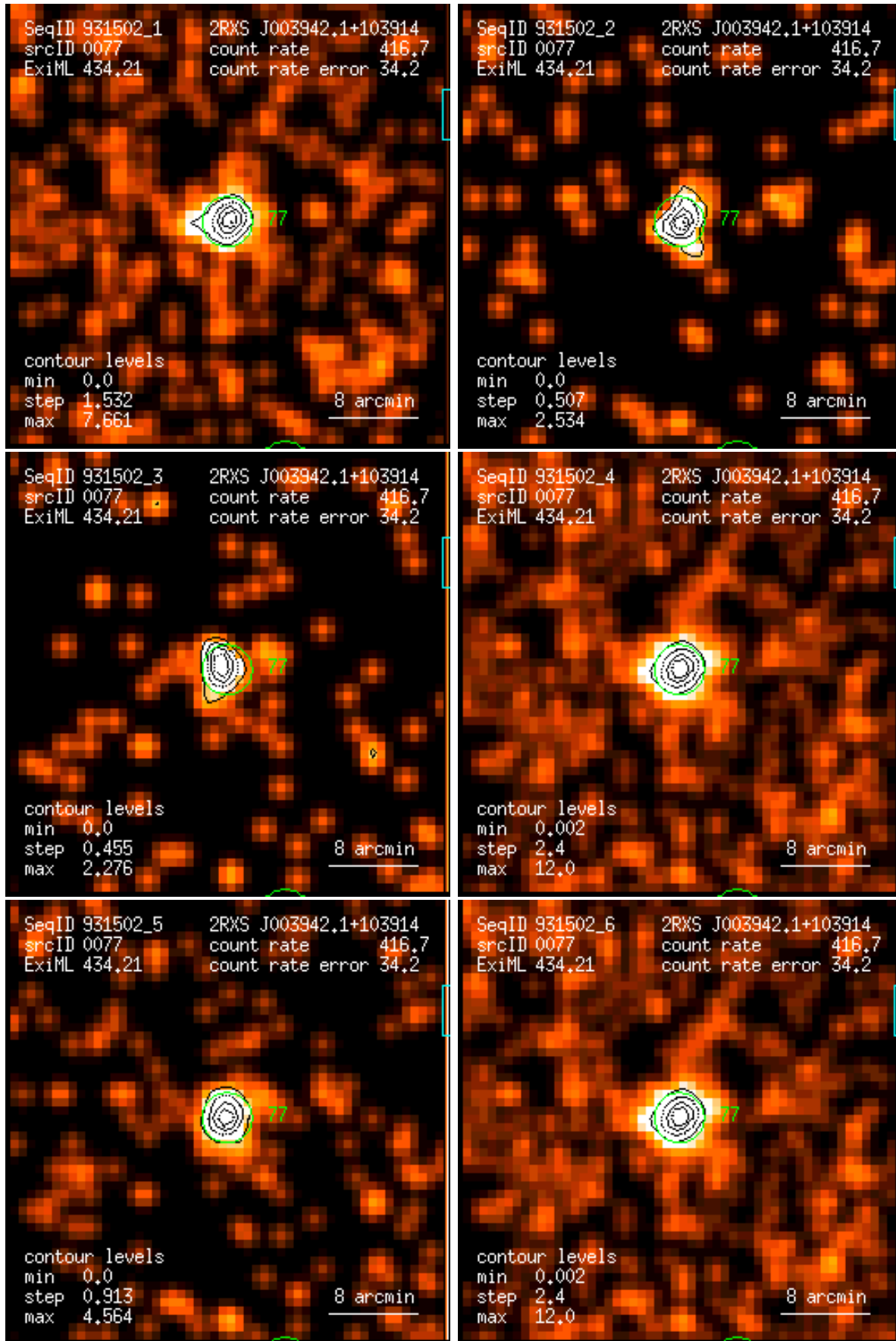
Figure 77: RASS 931502: detection 0077: band rate images, Gaussian filter: (1) PSPC channels 11 – 41, (2) 52 – 90, (3) 91 – 201, (4) 11 – 235, (5) 52 – 201, (6) 11 – 201. Broad band rates in counts/ks. Band rate contour levels in counts/ks/arcmin 2 .
