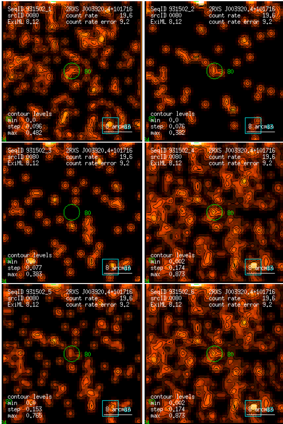
Figure 80: RASS 931502: detection 0080: band rate images, Gaussian filter: (1) PSPC channels 11 – 41, (2) 52 – 90, (3) 91 – 201, (4) 11 – 235, (5) 52 – 201, (6) 11 – 201. Broad band rates in counts/ks. Band rate contour levels in counts/ks/arcmin 2 .
