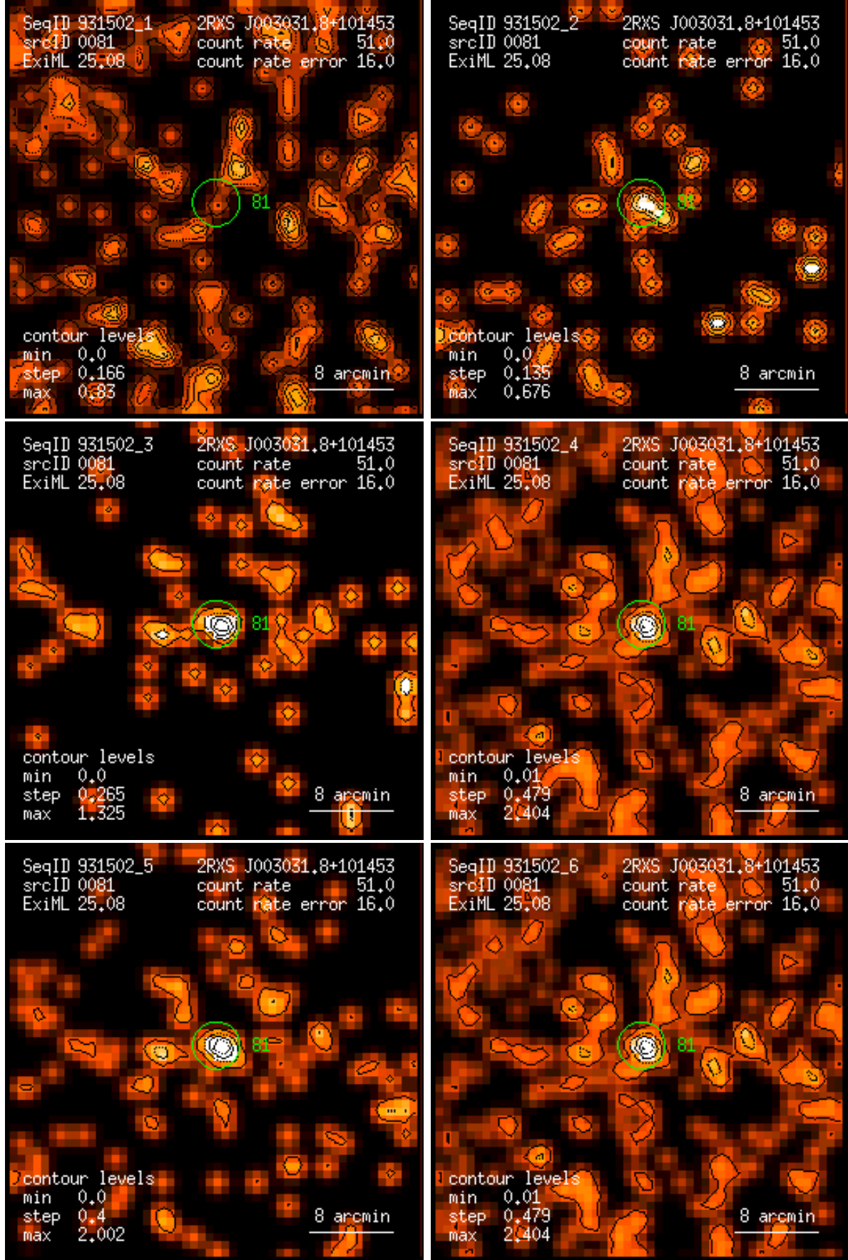
Figure 81: RASS 931502: detection 0081: band rate images, Gaussian filter: (1) PSPC channels 11 – 41, (2) 52 – 90, (3) 91 – 201, (4) 11 – 235, (5) 52 – 201, (6) 11 – 201. Broad band rates in counts/ks. Band rate contour levels in counts/ks/arcmin 2 .
