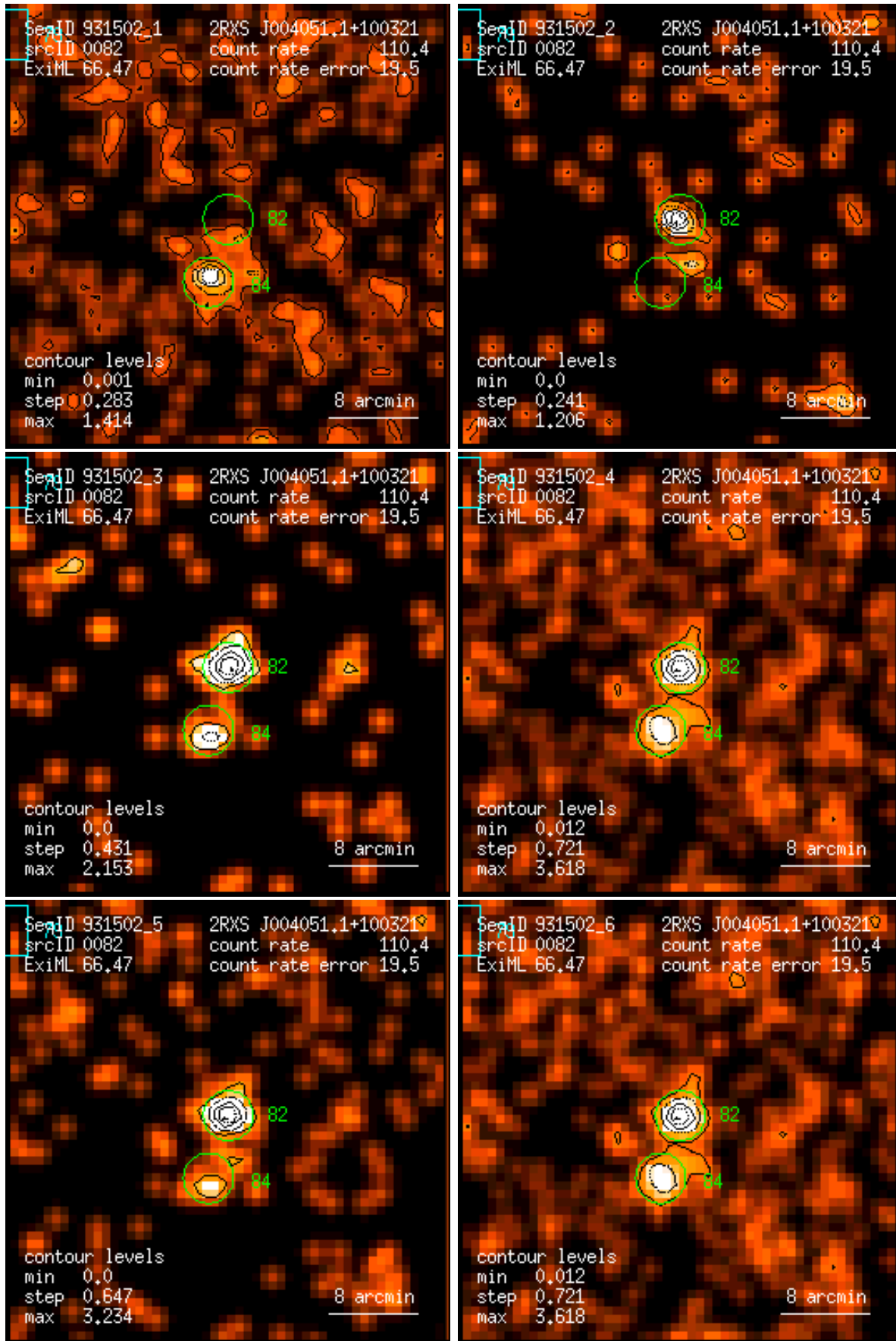
Figure 82: RASS 931502: detection 0082: band rate images, Gaussian filter: (1) PSPC channels 11 – 41, (2) 52 – 90, (3) 91 – 201, (4) 11 – 235, (5) 52 – 201, (6) 11 – 201. Broad band rates in counts/ks. Band rate contour levels in counts/ks/arcmin 2 .
