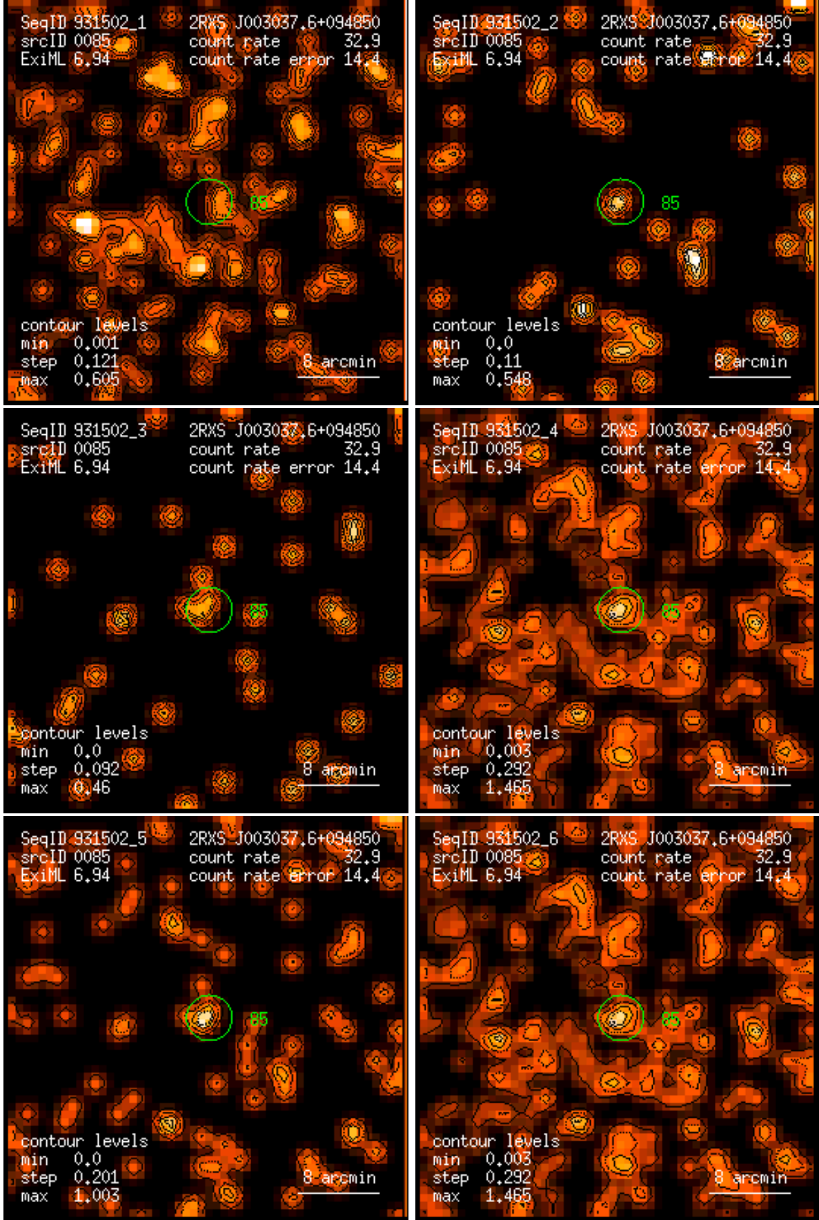
Figure 85: RASS 931502: detection 0085: band rate images, Gaussian filter: (1) PSPC channels 11 – 41, (2) 52 – 90, (3) 91 – 201, (4) 11 – 235, (5) 52 – 201, (6) 11 – 201. Broad band rates in counts/ks. Band rate contour levels in counts/ks/arcmin 2 .
