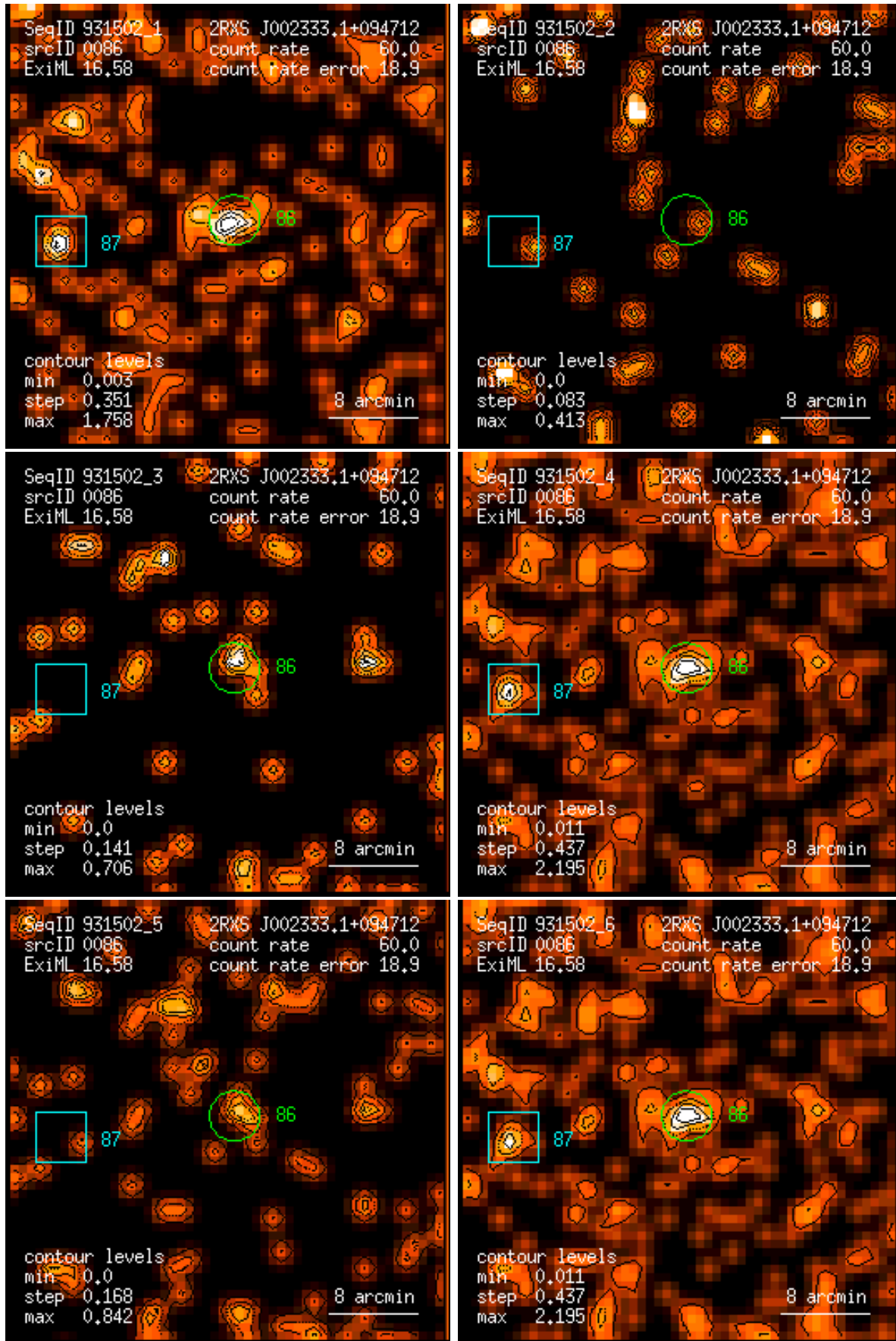
Figure 86: RASS 931502: detection 0086: band rate images, Gaussian filter: (1) PSPC channels 11 – 41, (2) 52 – 90, (3) 91 – 201, (4) 11 – 235, (5) 52 – 201, (6) 11 – 201. Broad band rates in counts/ks. Band rate contour levels in counts/ks/arcmin 2 .
