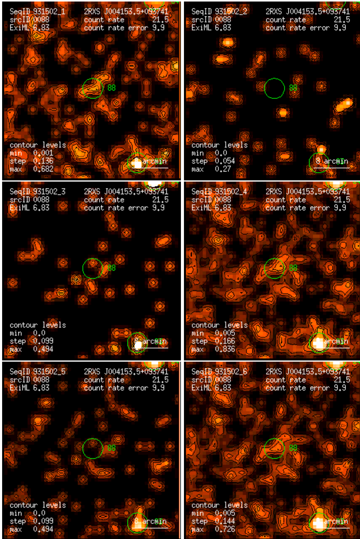
Figure 88: RASS 931502: detection 0088: band rate images, Gaussian filter: (1) PSPC channels 11 – 41, (2) 52 – 90, (3) 91 – 201, (4) 11 – 235, (5) 52 – 201, (6) 11 – 201. Broad band rates in counts/ks. Band rate contour levels in counts/ks/arcmin 2 .
