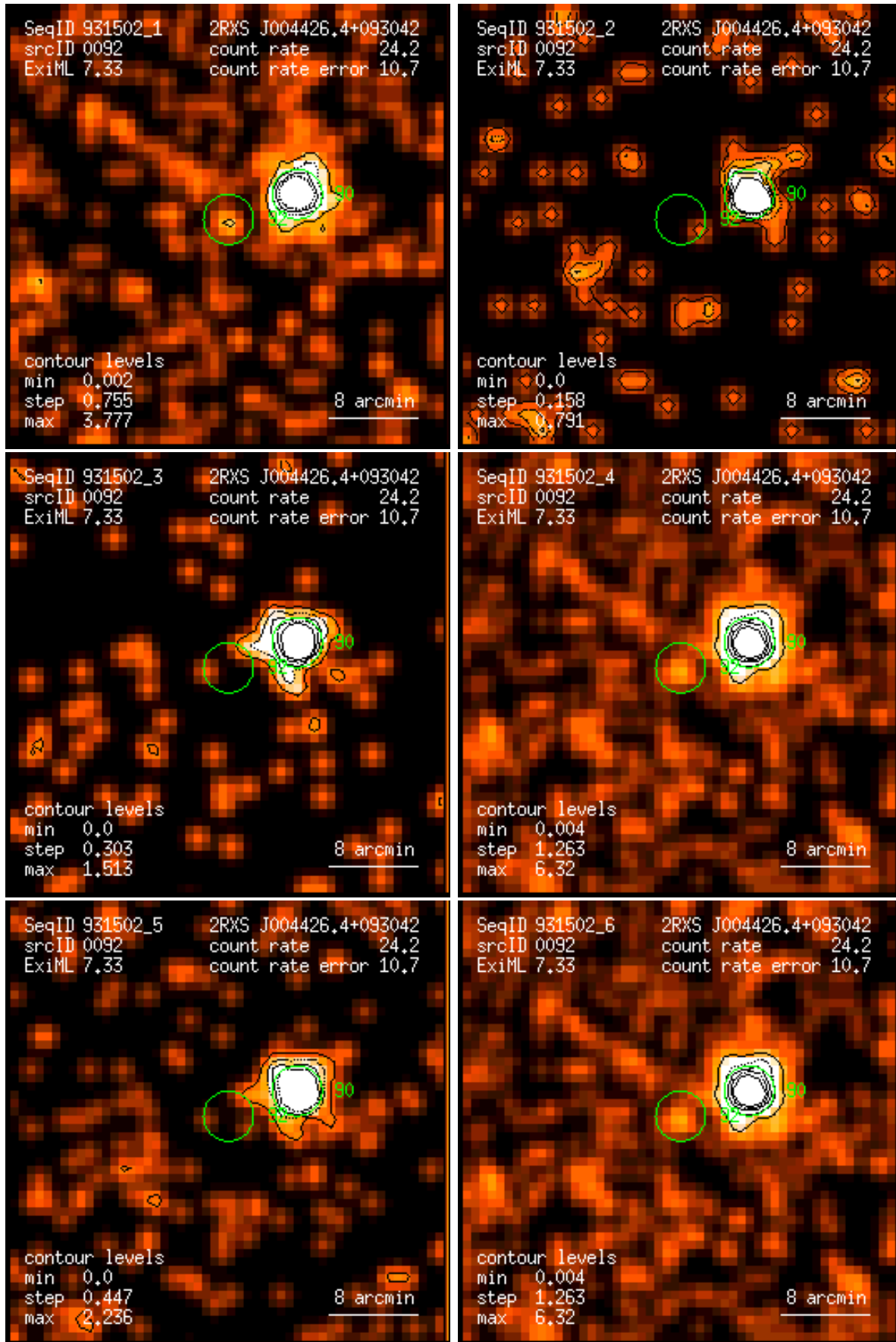
Figure 92: RASS 931502: detection 0092: band rate images, Gaussian filter: (1) PSPC channels 11 – 41, (2) 52 – 90, (3) 91 – 201, (4) 11 – 235, (5) 52 – 201, (6) 11 – 201. Broad band rates in counts/ks. Band rate contour levels in counts/ks/arcmin 2 .
