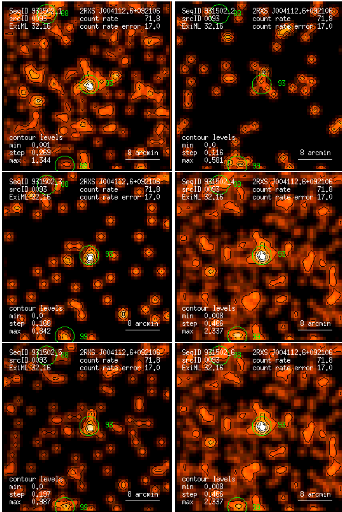
Figure 93: RASS 931502: detection 0093: band rate images, Gaussian filter: (1) PSPC channels 11 – 41, (2) 52 – 90, (3) 91 – 201, (4) 11 – 235, (5) 52 – 201, (6) 11 – 201. Broad band rates in counts/ks. Band rate contour levels in counts/ks/arcmin 2 .
