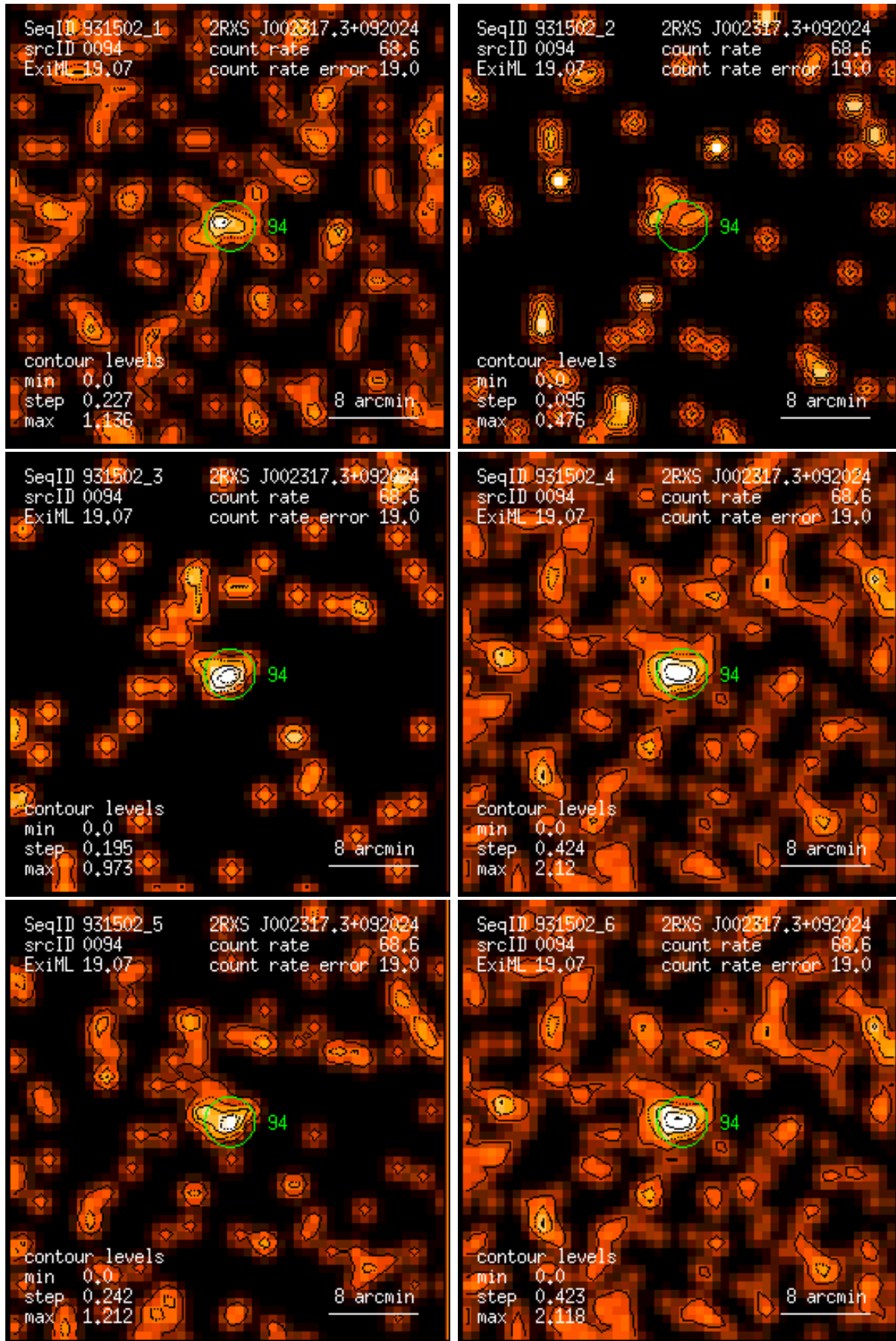
Figure 94: RASS 931502: detection 0094: band rate images, Gaussian filter: (1) PSPC channels 11 – 41, (2) 52 – 90, (3) 91 – 201, (4) 11 – 235, (5) 52 – 201, (6) 11 – 201. Broad band rates in counts/ks. Band rate contour levels in counts/ks/arcmin 2 .
