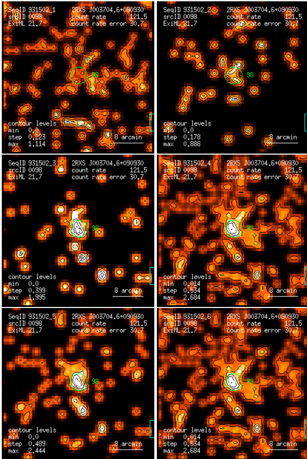
Figure 98: RASS 931502: detection 0098: band rate images, Gaussian filter: (1) PSPC channels 11 – 41, (2) 52 – 90, (3) 91 – 201, (4) 11 – 235, (5) 52 – 201, (6) 11 – 201. Broad band rates in counts/ks. Band rate contour levels in counts/ks/arcmin 2 .
