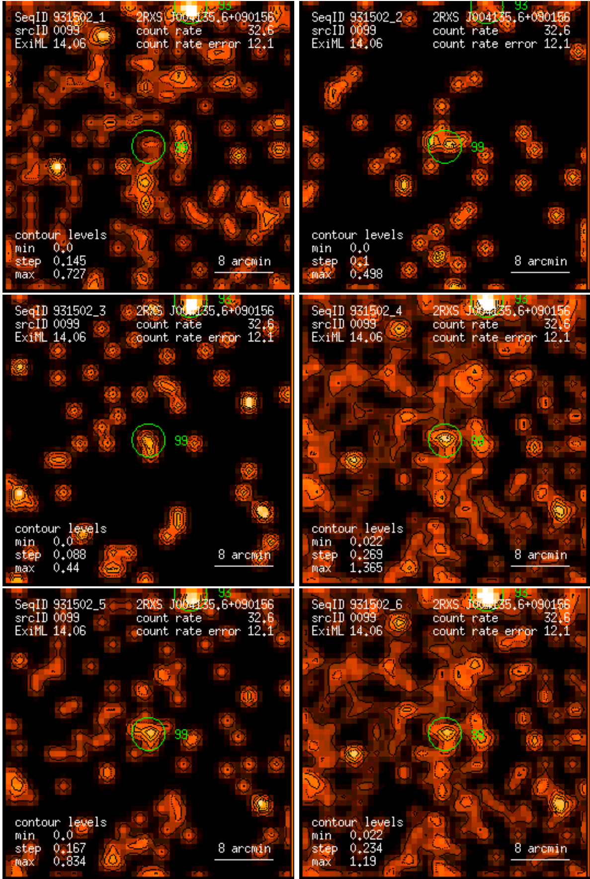
Figure 99: RASS 931502: detection 0099: band rate images, Gaussian filter: (1) PSPC channels 11 – 41, (2) 52 – 90, (3) 91 – 201, (4) 11 – 235, (5) 52 – 201, (6) 11 – 201. Broad band rates in counts/ks. Band rate contour levels in counts/ks/arcmin 2 .
