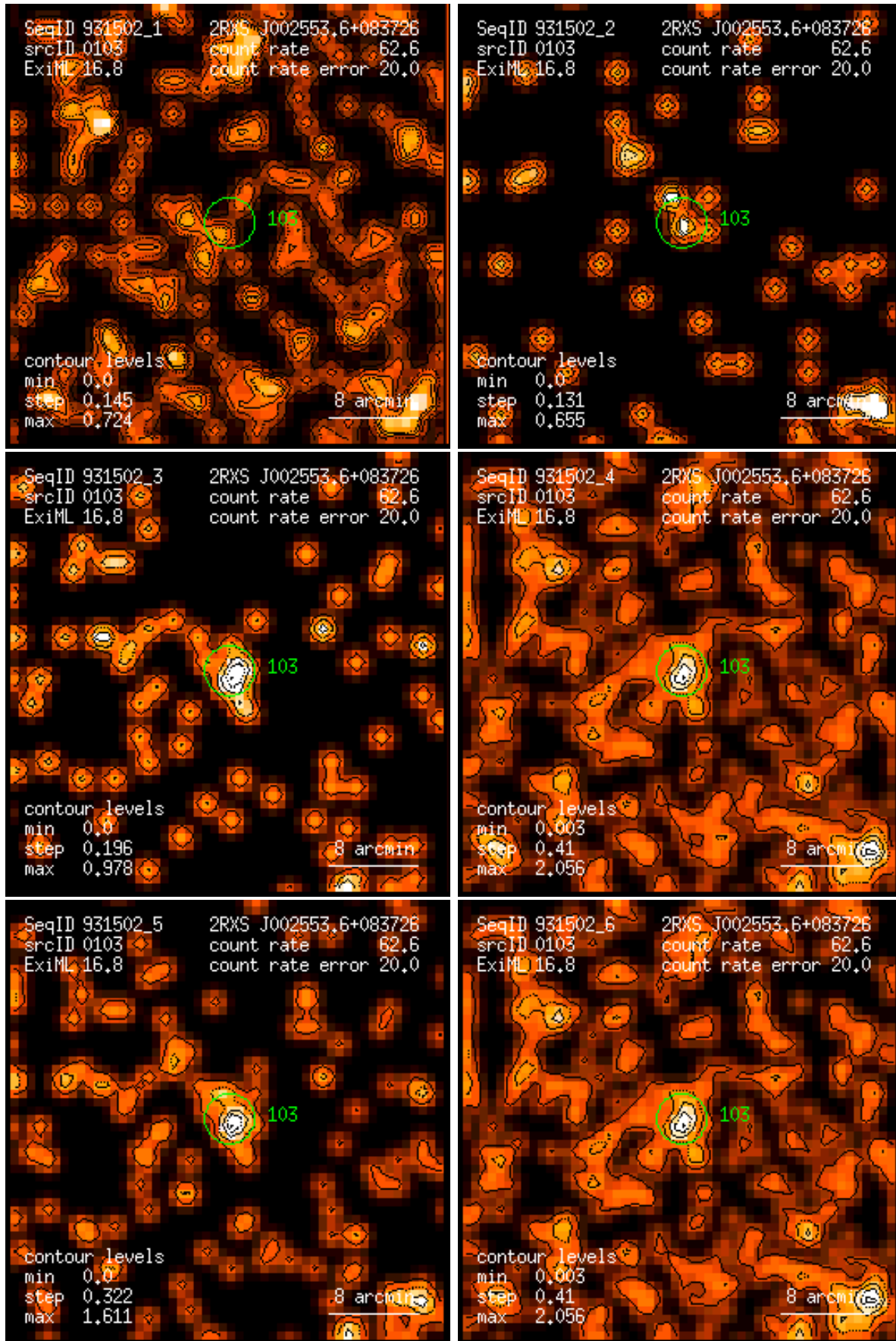
Figure 103: RASS 931502: detection 0103: band rate images, Gaussian filter: (1) PSPC channels 11 – 41, (2) 52 – 90, (3) 91 – 201, (4) 11 – 235, (5) 52 – 201, (6) 11 – 201. Broad band rates in counts/ks. Band rate contour levels in counts/ks/arcmin 2 .
