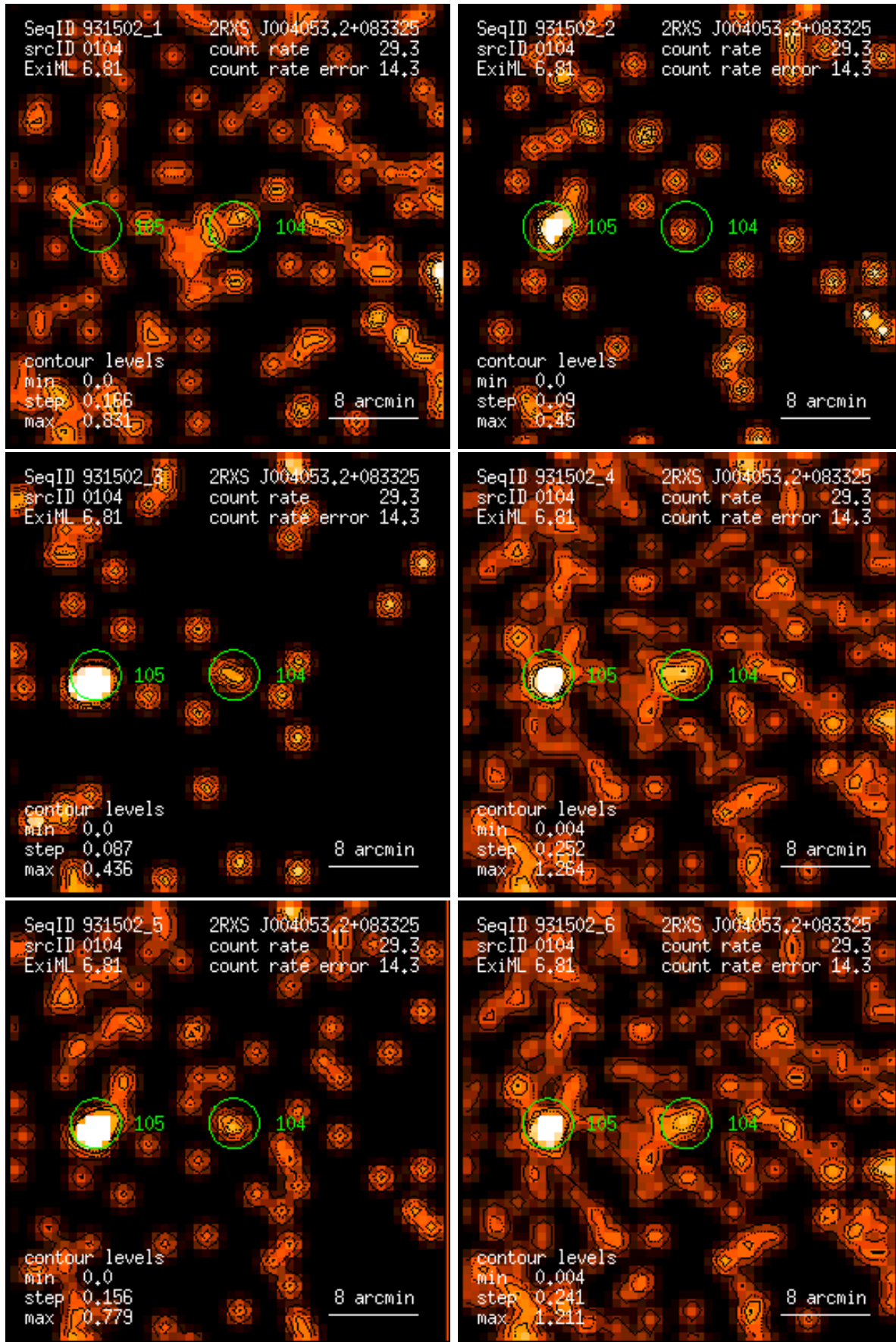
Figure 104: RASS 931502: detection 0104: band rate images, Gaussian filter: (1) PSPC channels 11 – 41, (2) 52 – 90, (3) 91 – 201, (4) 11 – 235, (5) 52 – 201, (6) 11 – 201. Broad band rates in counts/ks. Band rate contour levels in counts/ks/arcmin 2 .
