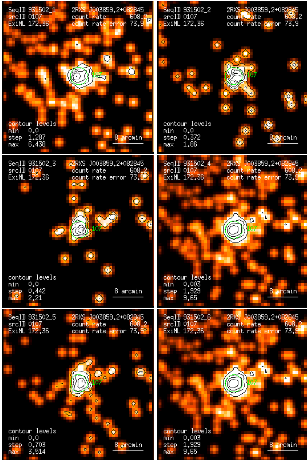
Figure 107: RASS 931502: detection 0107: band rate images, Gaussian filter: (1) PSPC channels 11 – 41, (2) 52 – 90, (3) 91 – 201, (4) 11 – 235, (5) 52 – 201, (6) 11 – 201. Broad band rates in counts/ks. Band rate contour levels in counts/ks/arcmin 2 .
