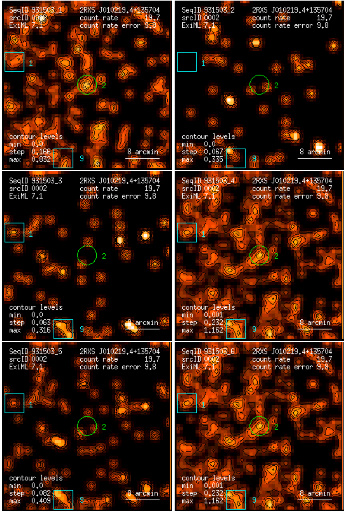
Figure 2: RASS 931503: detection 0002: band rate images, Gaussian filter: (1) PSPC channels 11 – 41, (2) 52 – 90, (3) 91 – 201, (4) 11 – 235, (5) 52 – 201, (6) 11 – 201. Broad band rates in counts/ks. Band rate contour levels in counts/ks/arcmin 2 .
