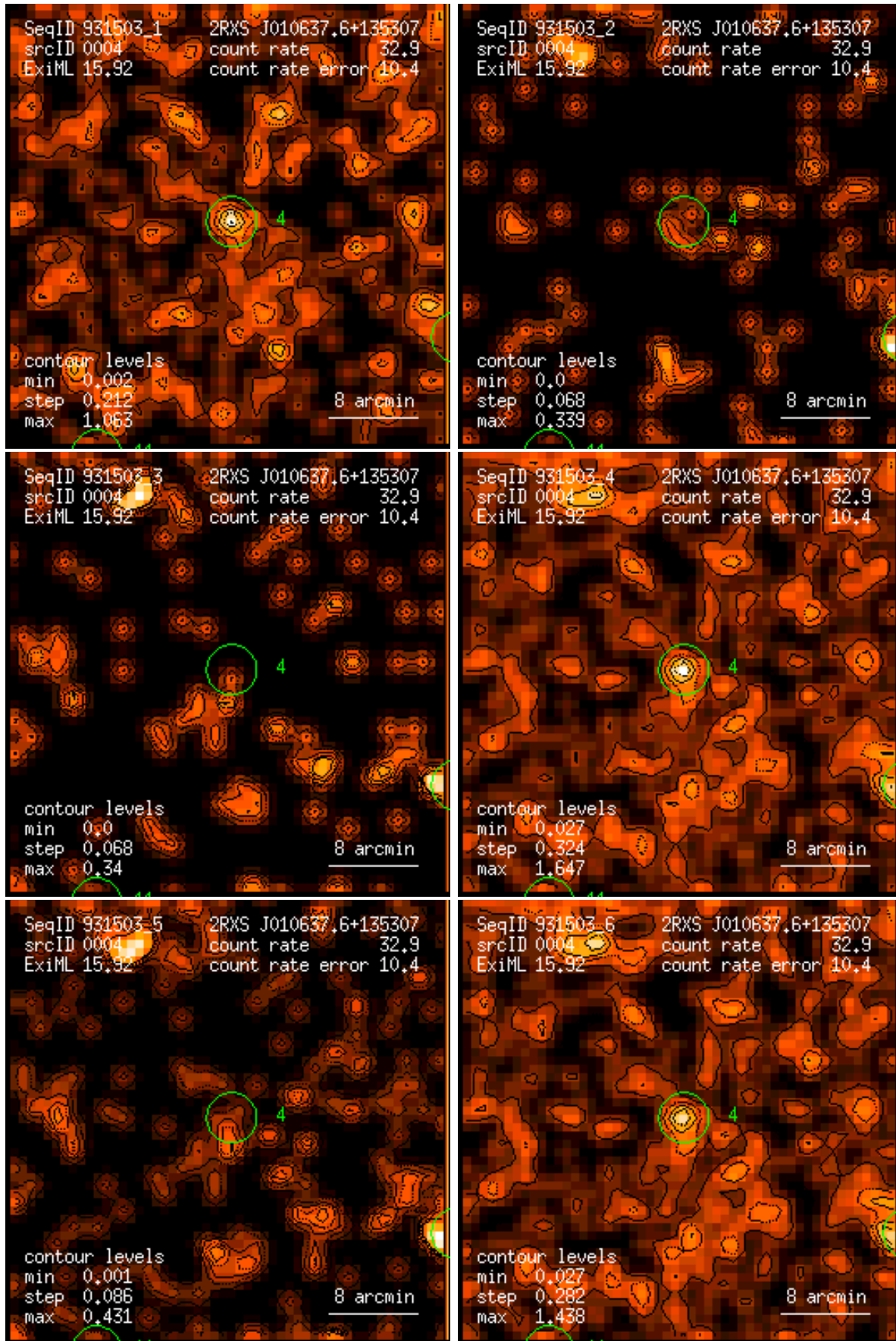
Figure 4: RASS 931503: detection 0004: band rate images, Gaussian filter: (1) PSPC channels 11 – 41, (2) 52 – 90, (3) 91 – 201, (4) 11 – 235, (5) 52 – 201, (6) 11 – 201. Broad band rates in counts/ks. Band rate contour levels in counts/ks/arcmin 2 .
