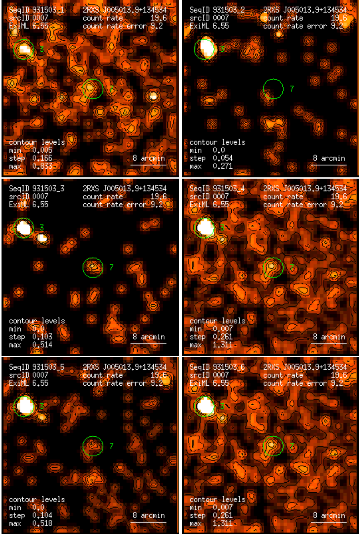
Figure 7: RASS 931503: detection 0007: band rate images, Gaussian filter: (1) PSPC channels 11 – 41, (2) 52 – 90, (3) 91 – 201, (4) 11 – 235, (5) 52 – 201, (6) 11 – 201. Broad band rates in counts/ks. Band rate contour levels in counts/ks/arcmin 2 .
