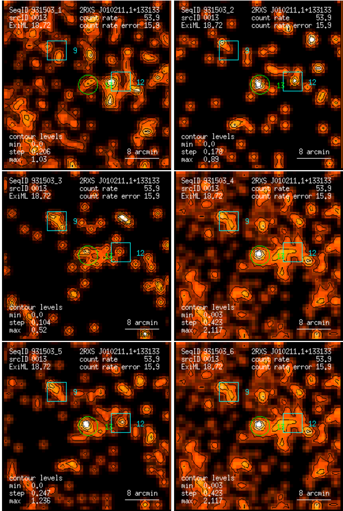
Figure 13: RASS 931503: detection 0013: band rate images, Gaussian filter: (1) PSPC channels 11 – 41, (2) 52 – 90, (3) 91 – 201, (4) 11 – 235, (5) 52 – 201, (6) 11 – 201. Broad band rates in counts/ks. Band rate contour levels in counts/ks/arcmin 2 .
