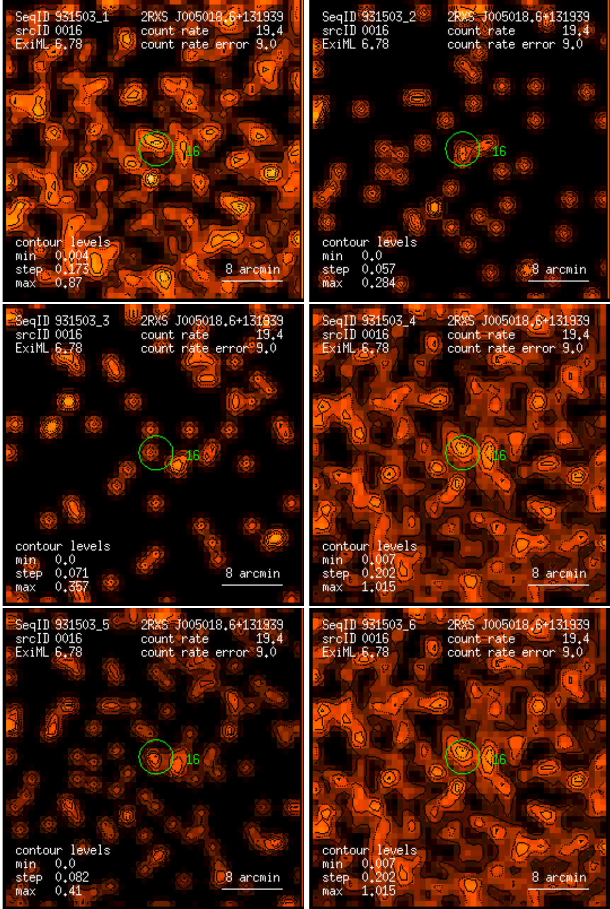
Figure 16: RASS 931503: detection 0016: band rate images, Gaussian filter: (1) PSPC channels 11 – 41, (2) 52 – 90, (3) 91 – 201, (4) 11 – 235, (5) 52 – 201, (6) 11 – 201. Broad band rates in counts/ks. Band rate contour levels in counts/ks/arcmin 2 .
