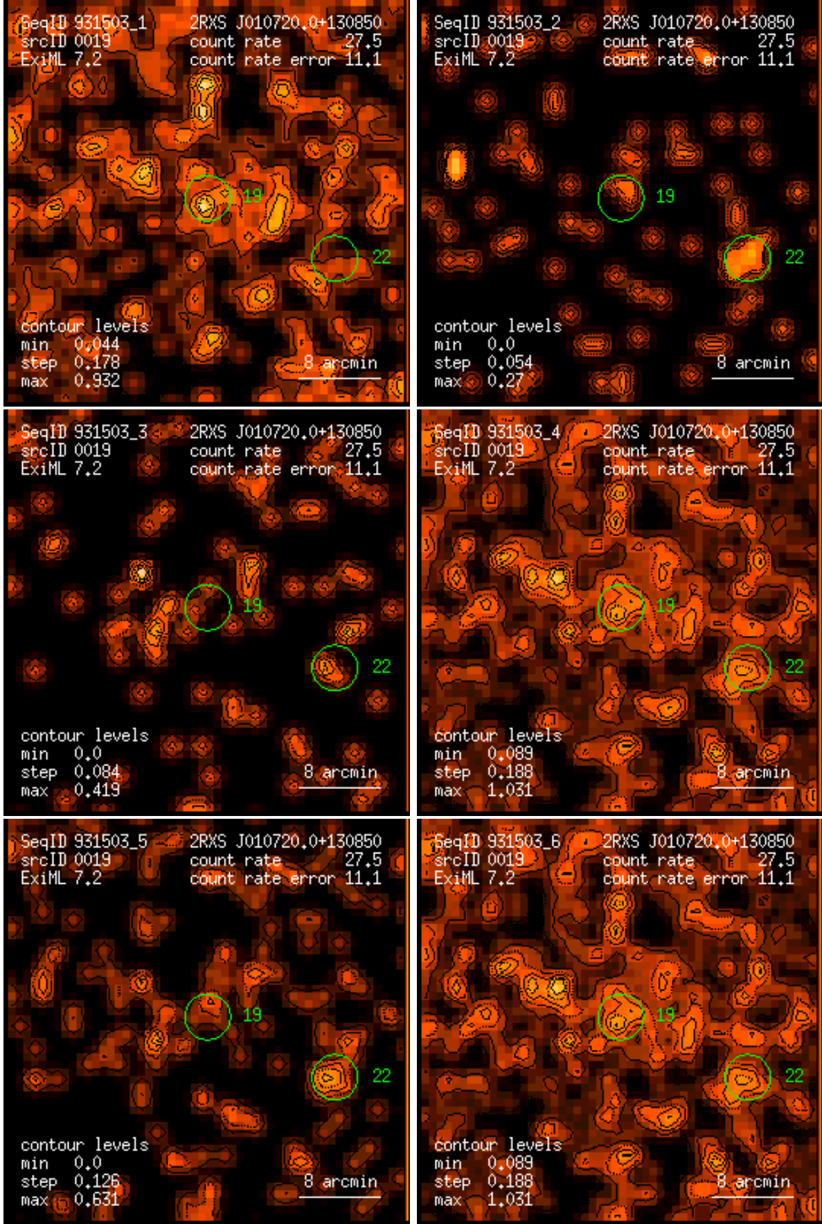
Figure 19: RASS 931503: detection 0019: band rate images, Gaussian filter: (1) PSPC channels 11 – 41, (2) 52 – 90, (3) 91 – 201, (4) 11 – 235, (5) 52 – 201, (6) 11 – 201. Broad band rates in counts/ks. Band rate contour levels in counts/ks/arcmin 2 .
