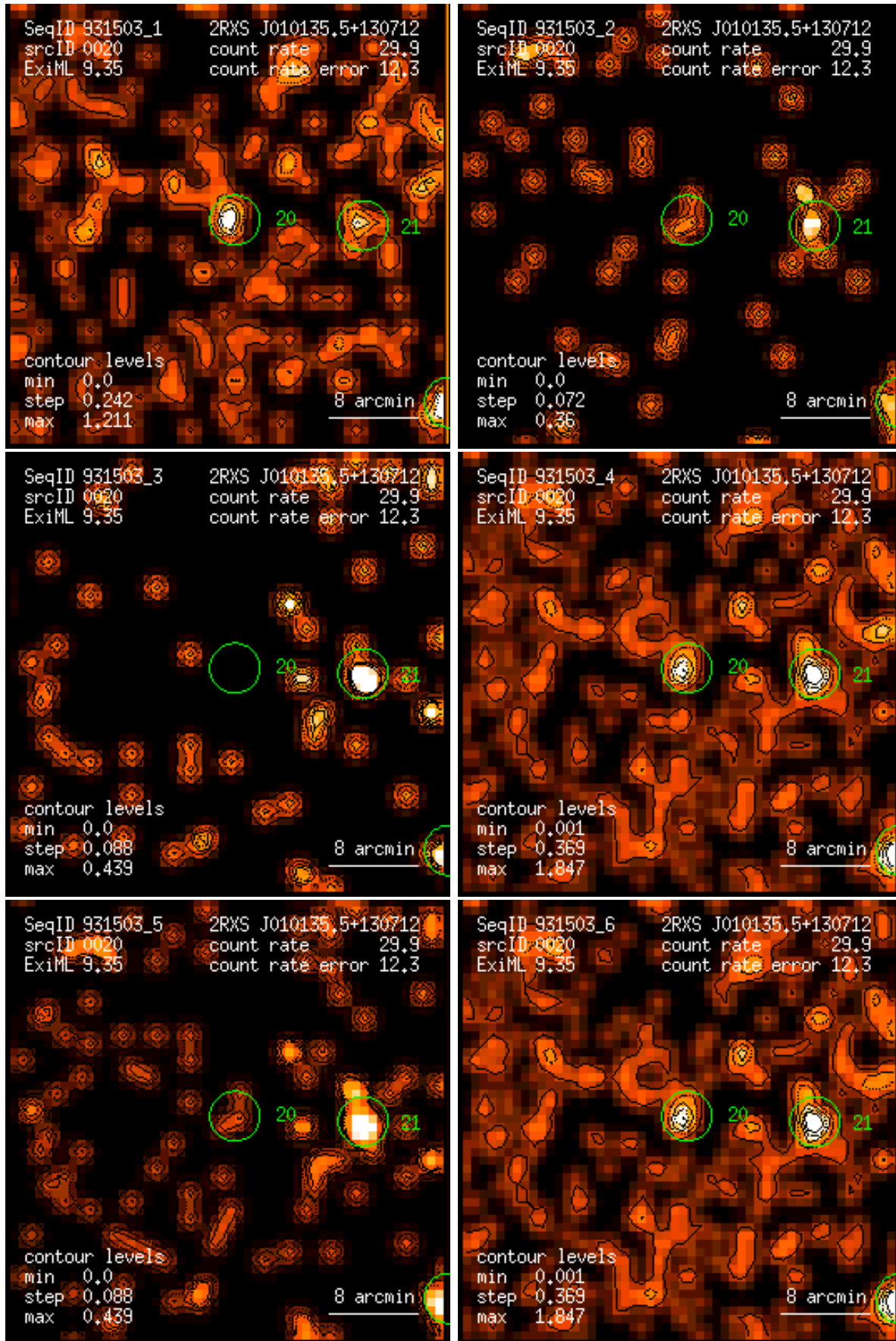
Figure 20: RASS 931503: detection 0020: band rate images, Gaussian filter: (1) PSPC channels 11 – 41, (2) 52 – 90, (3) 91 – 201, (4) 11 – 235, (5) 52 – 201, (6) 11 – 201. Broad band rates in counts/ks. Band rate contour levels in counts/ks/arcmin 2 .
