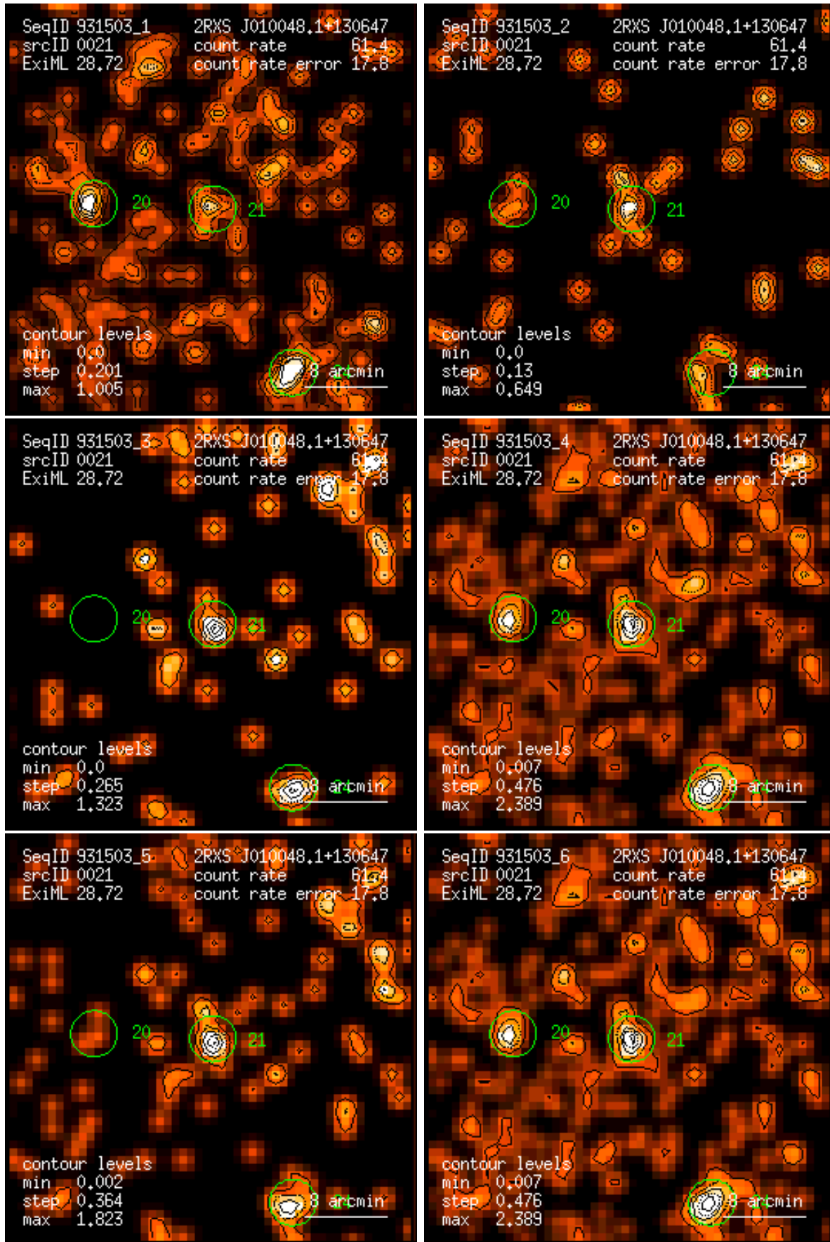
Figure 21: RASS 931503: detection 0021: band rate images, Gaussian filter: (1) PSPC channels 11 – 41, (2) 52 – 90, (3) 91 – 201, (4) 11 – 235, (5) 52 – 201, (6) 11 – 201. Broad band rates in counts/ks. Band rate contour levels in counts/ks/arcmin 2 .
