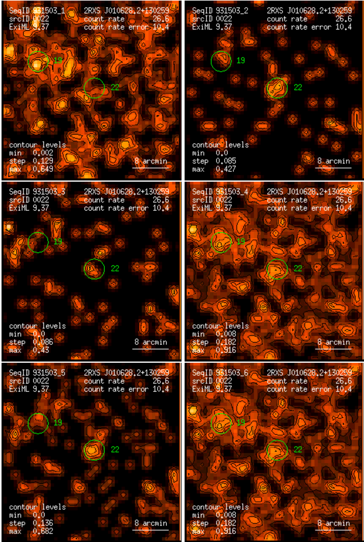
Figure 22: RASS 931503: detection 0022: band rate images, Gaussian filter: (1) PSPC channels 11 – 41, (2) 52 – 90, (3) 91 – 201, (4) 11 – 235, (5) 52 – 201, (6) 11 – 201. Broad band rates in counts/ks. Band rate contour levels in counts/ks/arcmin 2 .
