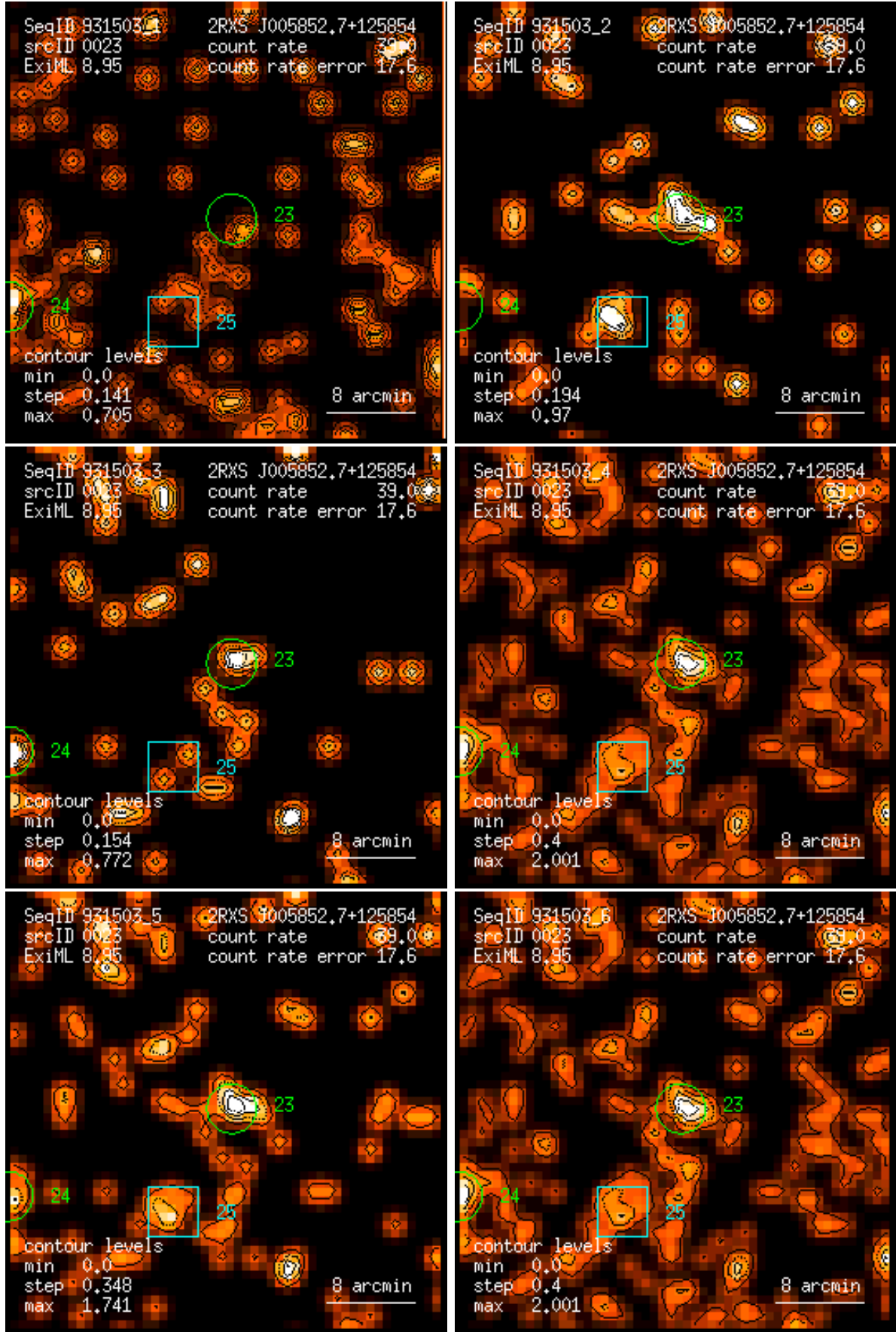
Figure 23: RASS 931503: detection 0023: band rate images, Gaussian filter: (1) PSPC channels 11 – 41, (2) 52 – 90, (3) 91 – 201, (4) 11 – 235, (5) 52 – 201, (6) 11 – 201. Broad band rates in counts/ks. Band rate contour levels in counts/ks/arcmin 2 .
