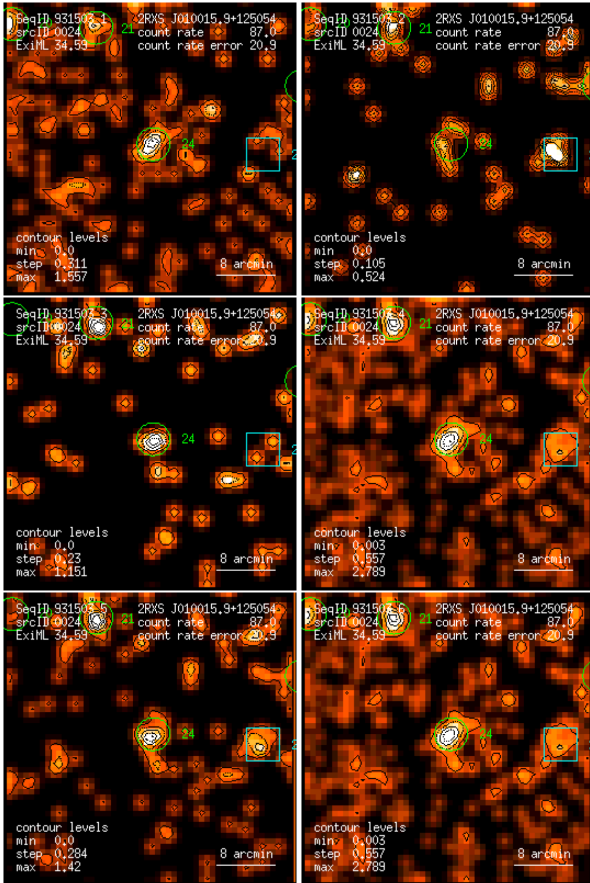
Figure 24: RASS 931503: detection 0024: band rate images, Gaussian filter: (1) PSPC channels 11 – 41, (2) 52 – 90, (3) 91 – 201, (4) 11 – 235, (5) 52 – 201, (6) 11 – 201. Broad band rates in counts/ks. Band rate contour levels in counts/ks/arcmin 2 .
