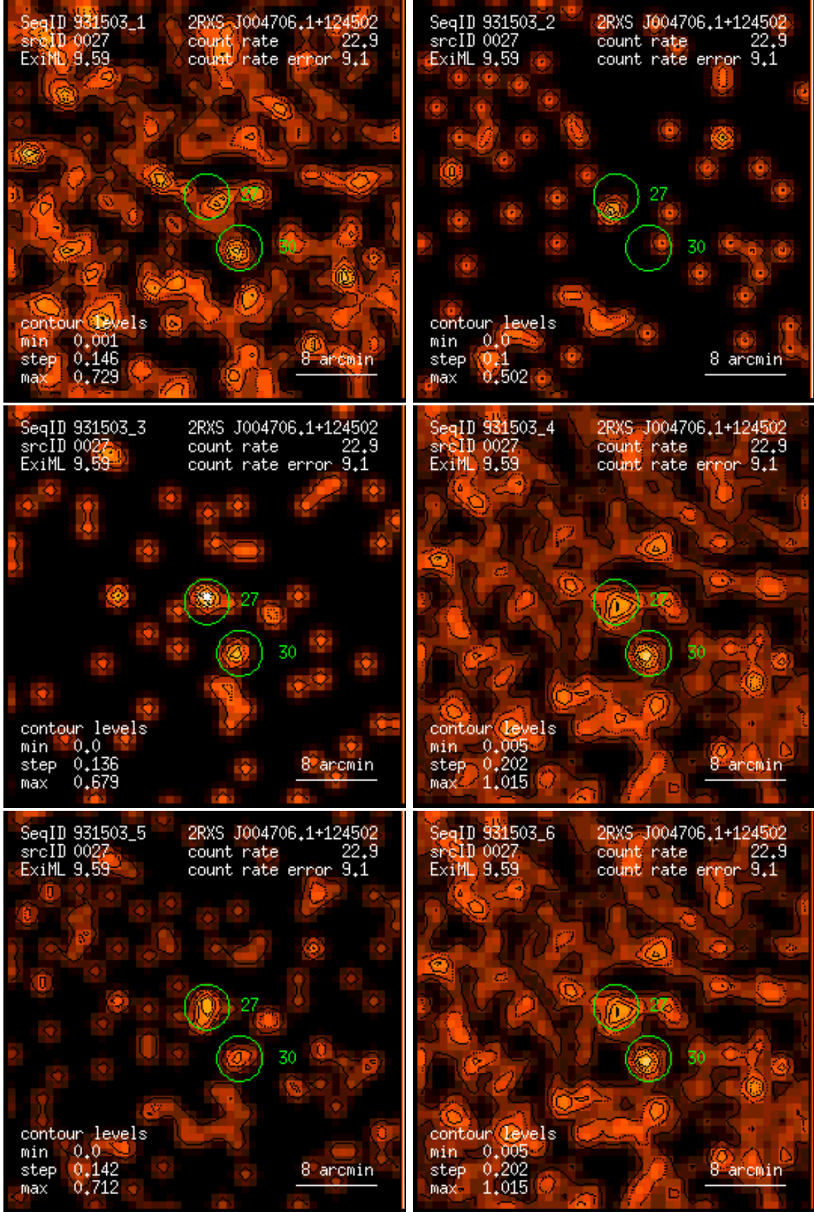
Figure 27: RASS 931503: detection 0027: band rate images, Gaussian filter: (1) PSPC channels 11 – 41, (2) 52 – 90, (3) 91 – 201, (4) 11 – 235, (5) 52 – 201, (6) 11 – 201. Broad band rates in counts/ks. Band rate contour levels in counts/ks/arcmin 2 .
